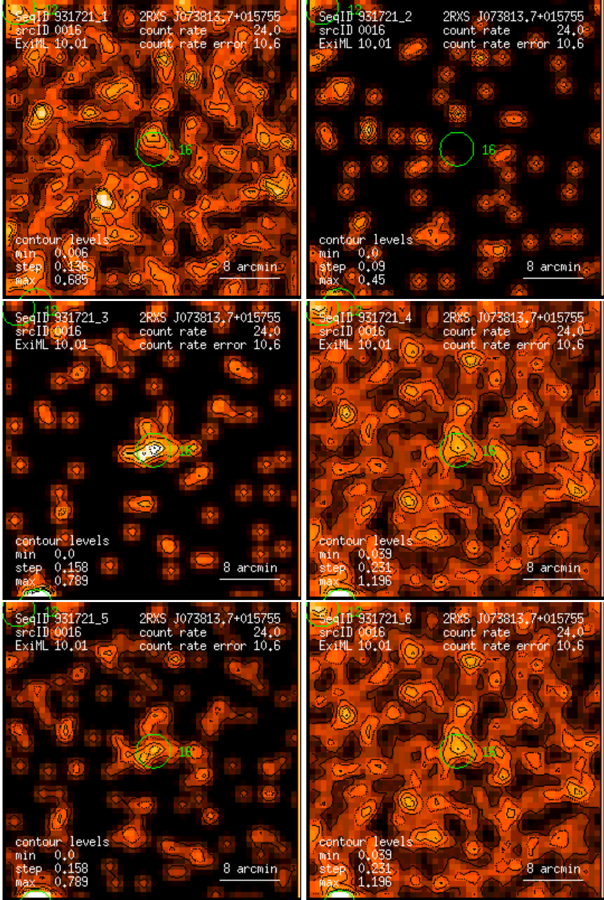
Figure 16: RASS 931721: detection 0016: band rate images, Gaussian filter: (1) PSPC channels 11 – 41, (2) 52 – 90, (3) 91 – 201, (4) 11 – 235, (5) 52 – 201, (6) 11 – 201. Broad band rates in counts/ks. Band rate contour levels in counts/ks/arcmin 2 .
