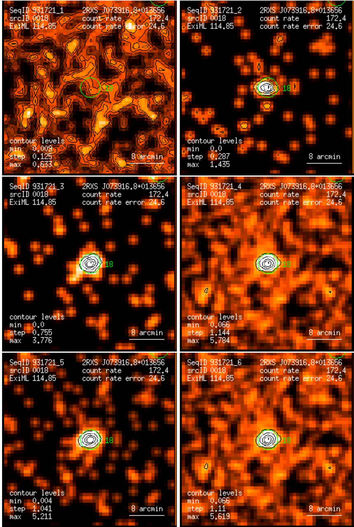
Figure 18: RASS 931721: detection 0018: band rate images, Gaussian filter: (1) PSPC channels 11 – 41, (2) 52 – 90, (3) 91 – 201, (4) 11 – 235, (5) 52 – 201, (6) 11 – 201. Broad band rates in counts/ks. Band rate contour levels in counts/ks/arcmin 2 .
