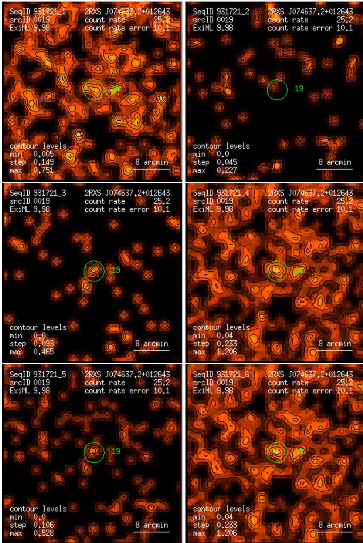
Figure 19: RASS 931721: detection 0019: band rate images, Gaussian filter: (1) PSPC channels 11 – 41, (2) 52 – 90, (3) 91 – 201, (4) 11 – 235, (5) 52 – 201, (6) 11 – 201. Broad band rates in counts/ks. Band rate contour levels in counts/ks/arcmin 2 .
