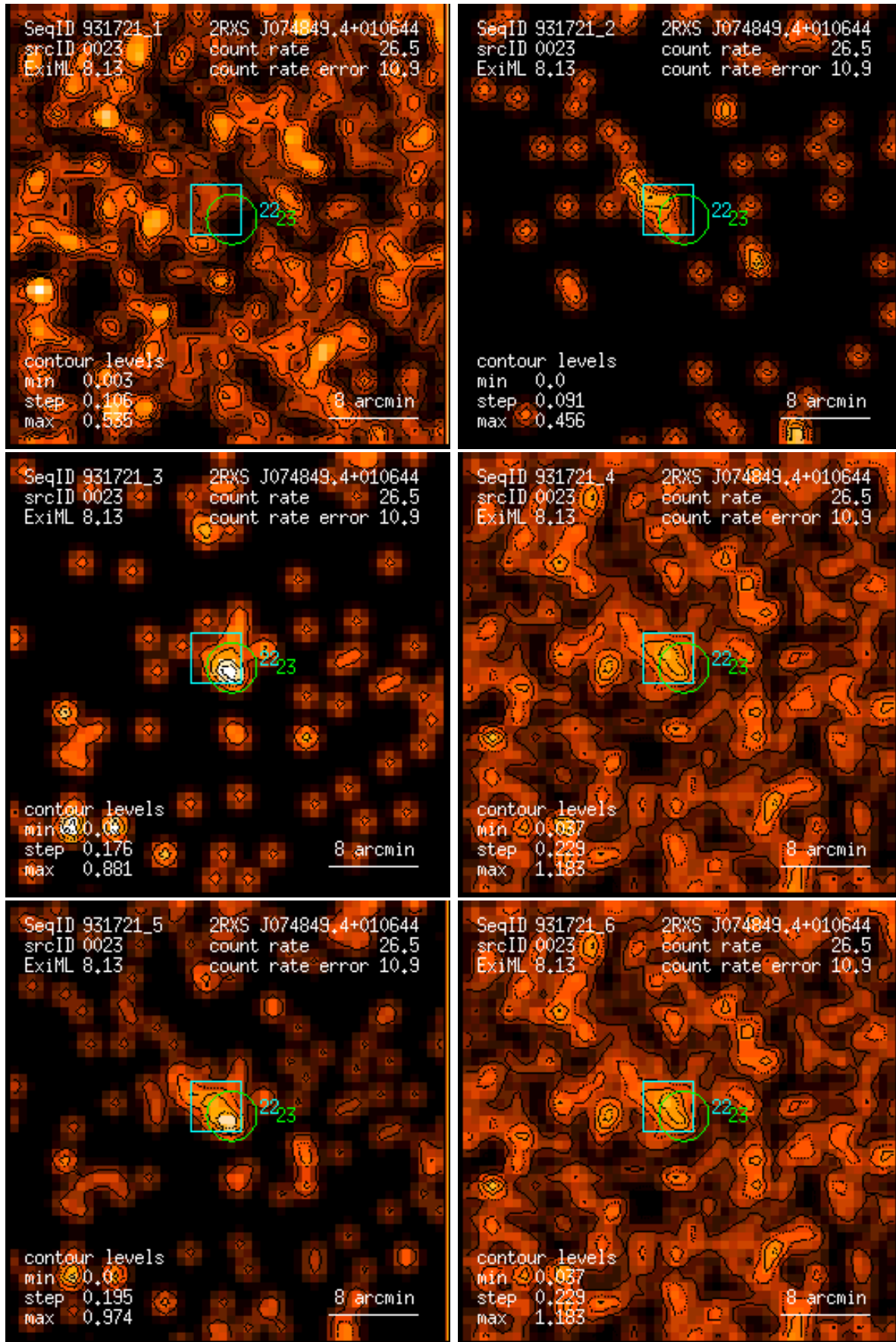
Figure 23: RASS 931721: detection 0023: band rate images, Gaussian filter: (1) PSPC channels 11 – 41, (2) 52 – 90, (3) 91 – 201, (4) 11 – 235, (5) 52 – 201, (6) 11 – 201. Broad band rates in counts/ks. Band rate contour levels in counts/ks/arcmin 2 .
