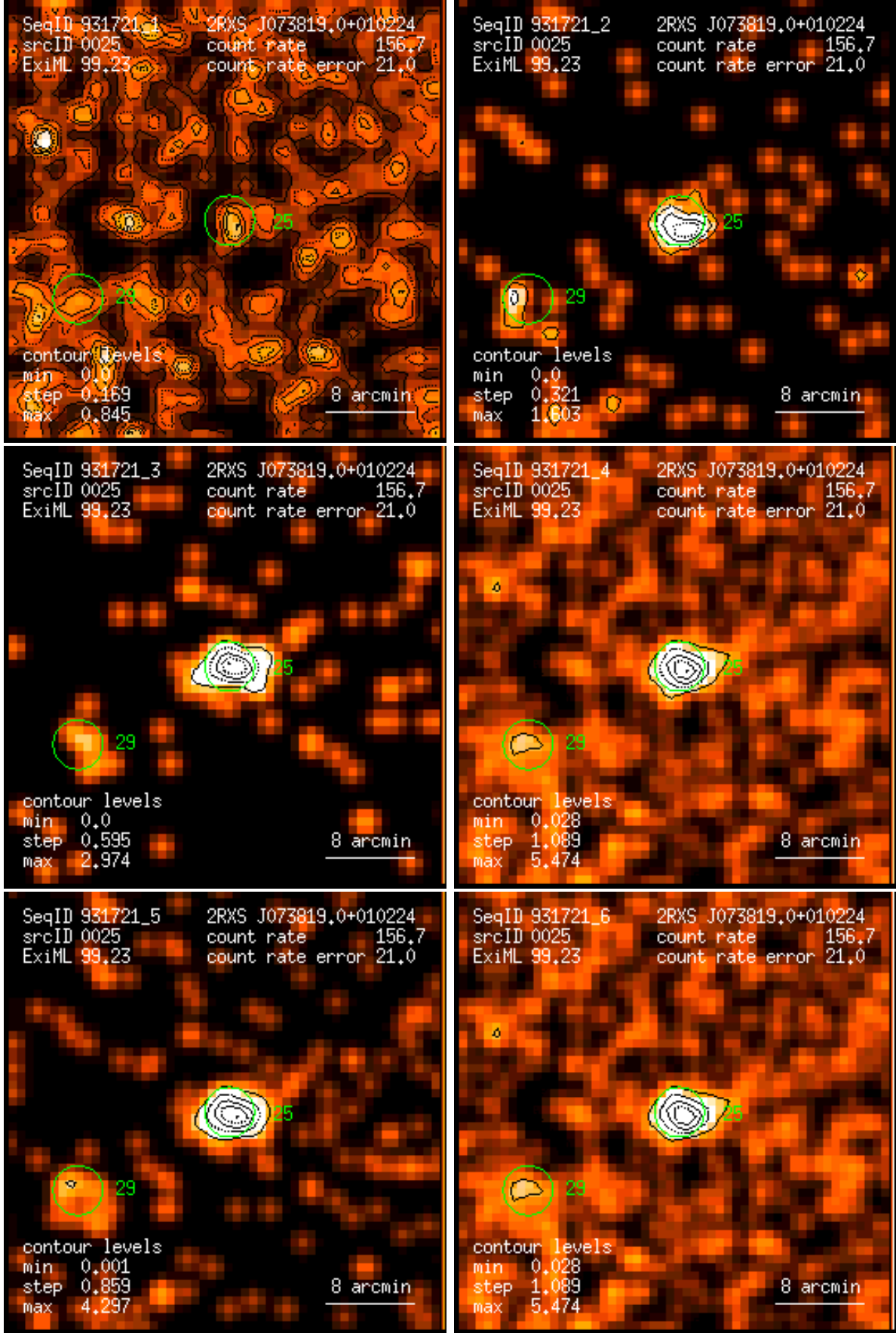
Figure 25: RASS 931721: detection 0025: band rate images, Gaussian filter: (1) PSPC channels 11 – 41, (2) 52 – 90, (3) 91 – 201, (4) 11 – 235, (5) 52 – 201, (6) 11 – 201. Broad band rates in counts/ks. Band rate contour levels in counts/ks/arcmin 2 .
