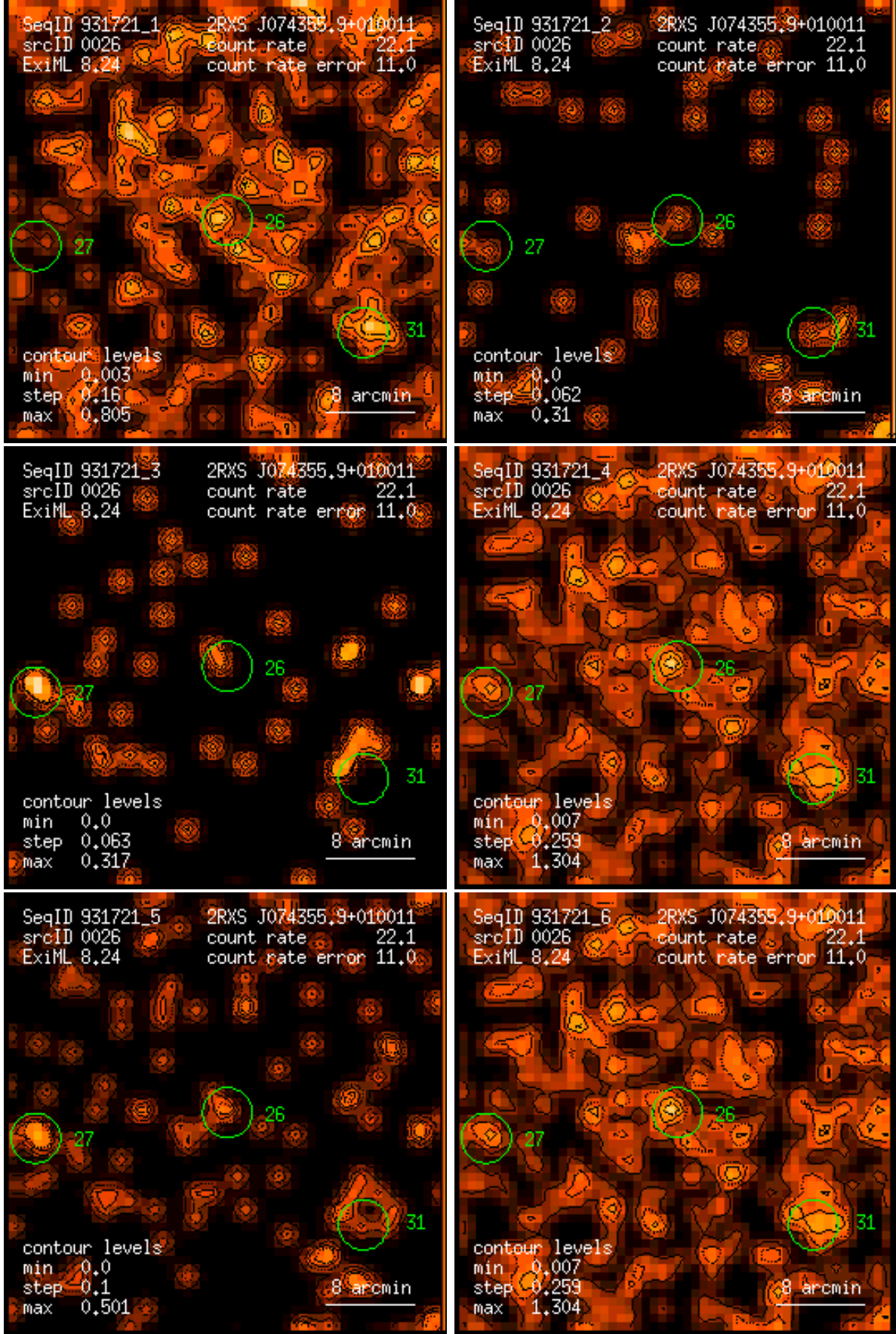
Figure 26: RASS 931721: detection 0026: band rate images, Gaussian filter: (1) PSPC channels 11 – 41, (2) 52 – 90, (3) 91 – 201, (4) 11 – 235, (5) 52 – 201, (6) 11 – 201. Broad band rates in counts/ks. Band rate contour levels in counts/ks/arcmin 2 .
