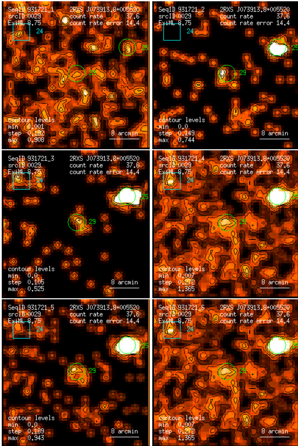
Figure 29: RASS 931721: detection 0029: band rate images, Gaussian filter: (1) PSPC channels 11 – 41, (2) 52 – 90, (3) 91 – 201, (4) 11 – 235, (5) 52 – 201, (6) 11 – 201. Broad band rates in counts/ks. Band rate contour levels in counts/ks/arcmin 2 .
