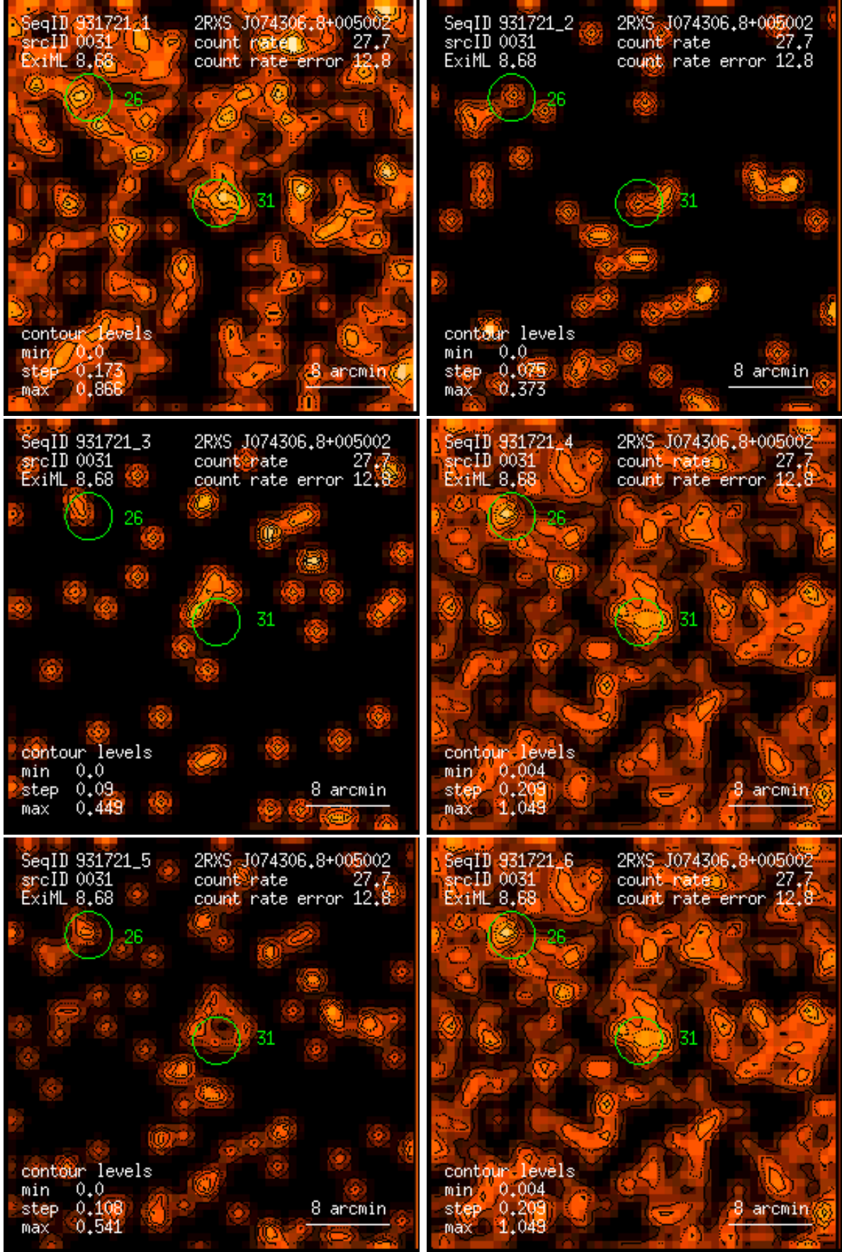
Figure 31: RASS 931721: detection 0031: band rate images, Gaussian filter: (1) PSPC channels 11 – 41, (2) 52 – 90, (3) 91 – 201, (4) 11 – 235, (5) 52 – 201, (6) 11 – 201. Broad band rates in counts/ks. Band rate contour levels in counts/ks/arcmin 2 .
