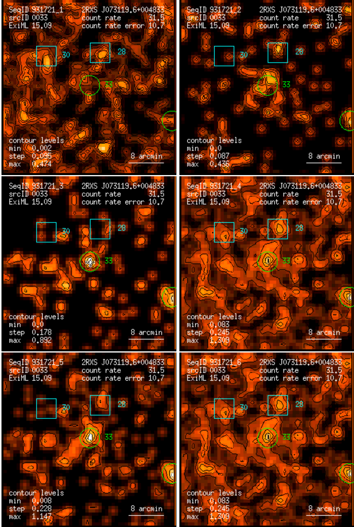
Figure 33: RASS 931721: detection 0033: band rate images, Gaussian filter: (1) PSPC channels 11 – 41, (2) 52 – 90, (3) 91 – 201, (4) 11 – 235, (5) 52 – 201, (6) 11 – 201. Broad band rates in counts/ks. Band rate contour levels in counts/ks/arcmin 2 .
