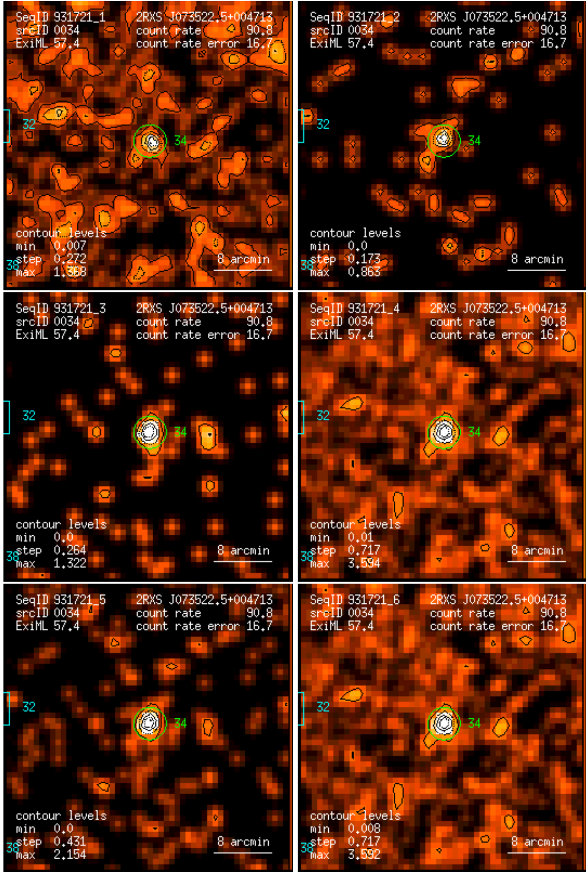
Figure 34: RASS 931721: detection 0034: band rate images, Gaussian filter: (1) PSPC channels 11 – 41, (2) 52 – 90, (3) 91 – 201, (4) 11 – 235, (5) 52 – 201, (6) 11 – 201. Broad band rates in counts/ks. Band rate contour levels in counts/ks/arcmin 2 .
