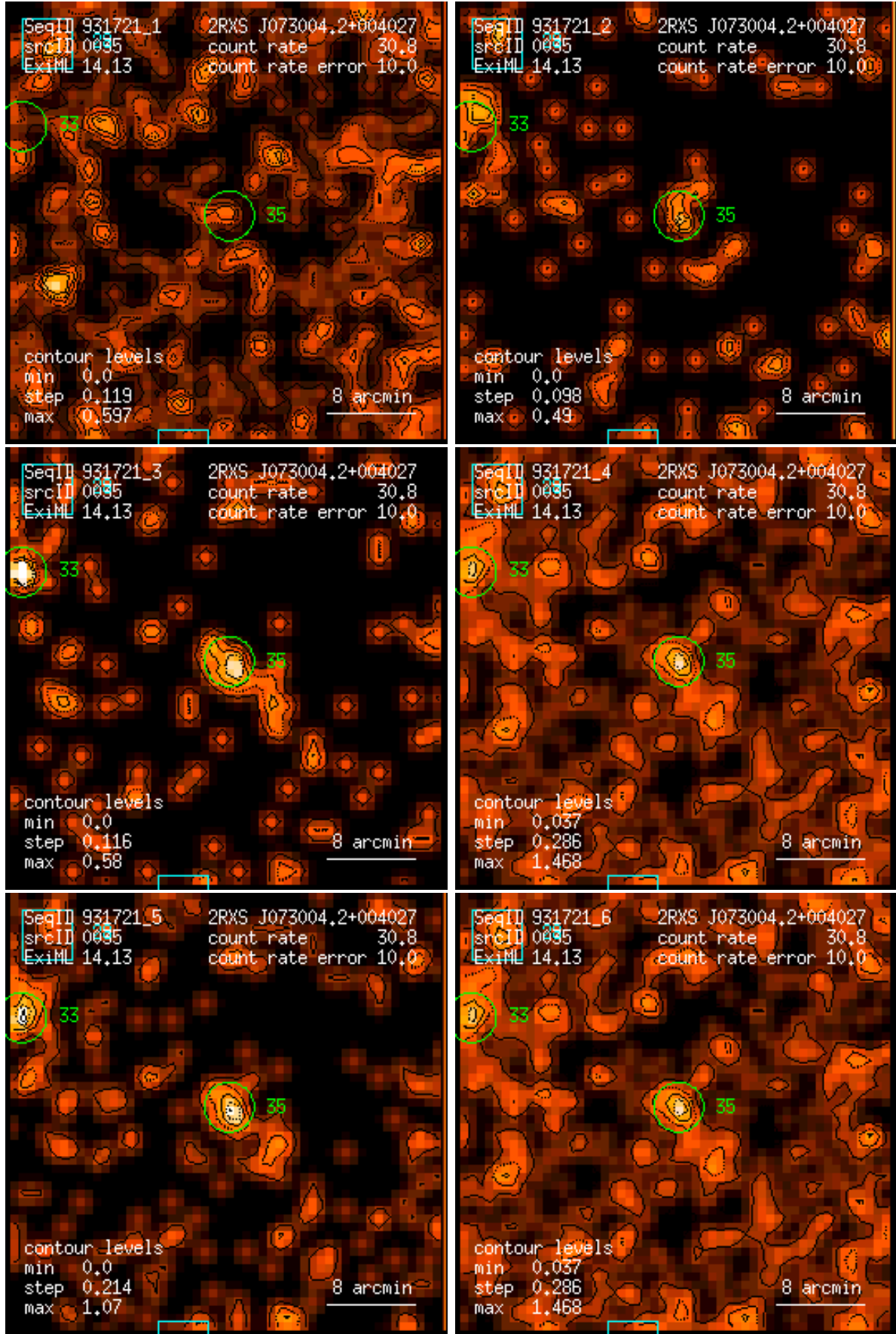
Figure 35: RASS 931721: detection 0035: band rate images, Gaussian filter: (1) PSPC channels 11 – 41, (2) 52 – 90, (3) 91 – 201, (4) 11 – 235, (5) 52 – 201, (6) 11 – 201. Broad band rates in counts/ks. Band rate contour levels in counts/ks/arcmin 2 .
