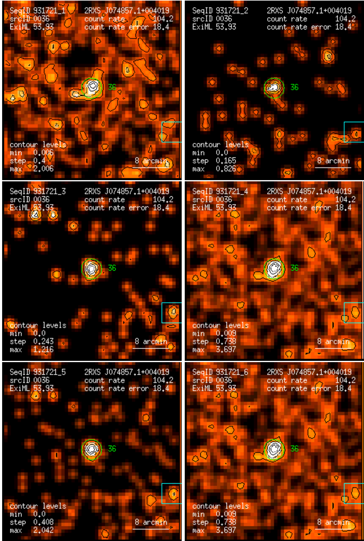
Figure 36: RASS 931721: detection 0036: band rate images, Gaussian filter: (1) PSPC channels 11 – 41, (2) 52 – 90, (3) 91 – 201, (4) 11 – 235, (5) 52 – 201, (6) 11 – 201. Broad band rates in counts/ks. Band rate contour levels in counts/ks/arcmin 2 .
