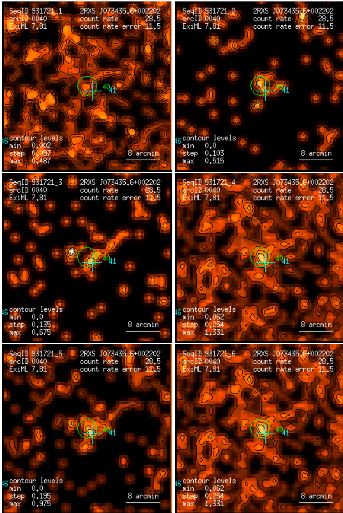
Figure 40: RASS 931721: detection 0040: band rate images, Gaussian filter: (1) PSPC channels 11 – 41, (2) 52 – 90, (3) 91 – 201, (4) 11 – 235, (5) 52 – 201, (6) 11 – 201. Broad band rates in counts/ks. Band rate contour levels in counts/ks/arcmin 2 .
