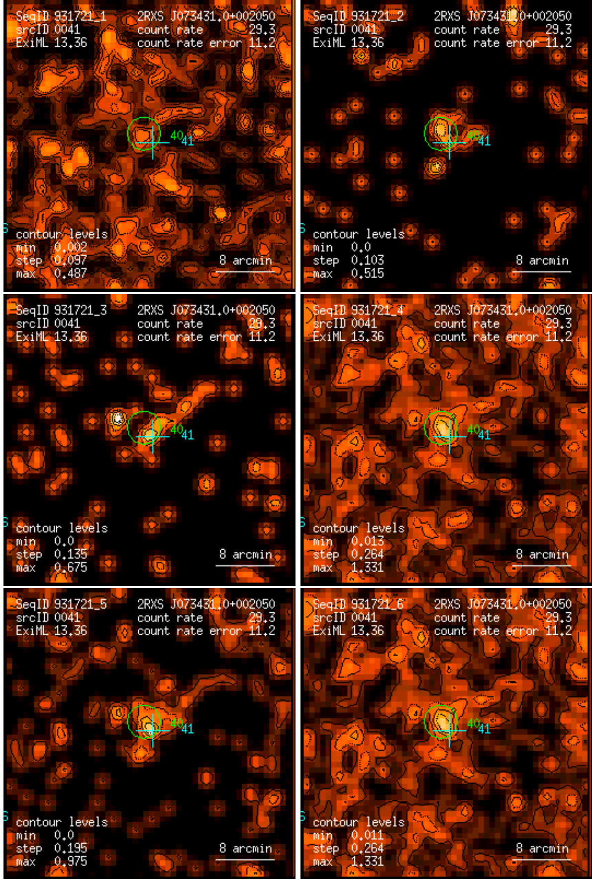
Figure 41: RASS 931721: detection 0041: band rate images, Gaussian filter: (1) PSPC channels 11 – 41, (2) 52 – 90, (3) 91 – 201, (4) 11 – 235, (5) 52 – 201, (6) 11 – 201. Broad band rates in counts/ks. Band rate contour levels in counts/ks/arcmin 2 .
