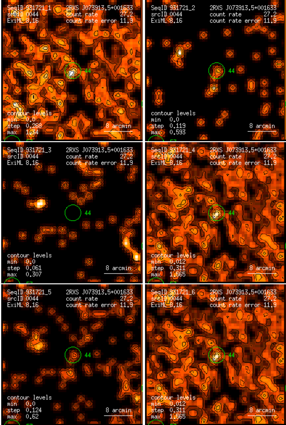
Figure 44: RASS 931721: detection 0044: band rate images, Gaussian filter: (1) PSPC channels 11 – 41, (2) 52 – 90, (3) 91 – 201, (4) 11 – 235, (5) 52 – 201, (6) 11 – 201. Broad band rates in counts/ks. Band rate contour levels in counts/ks/arcmin 2 .
