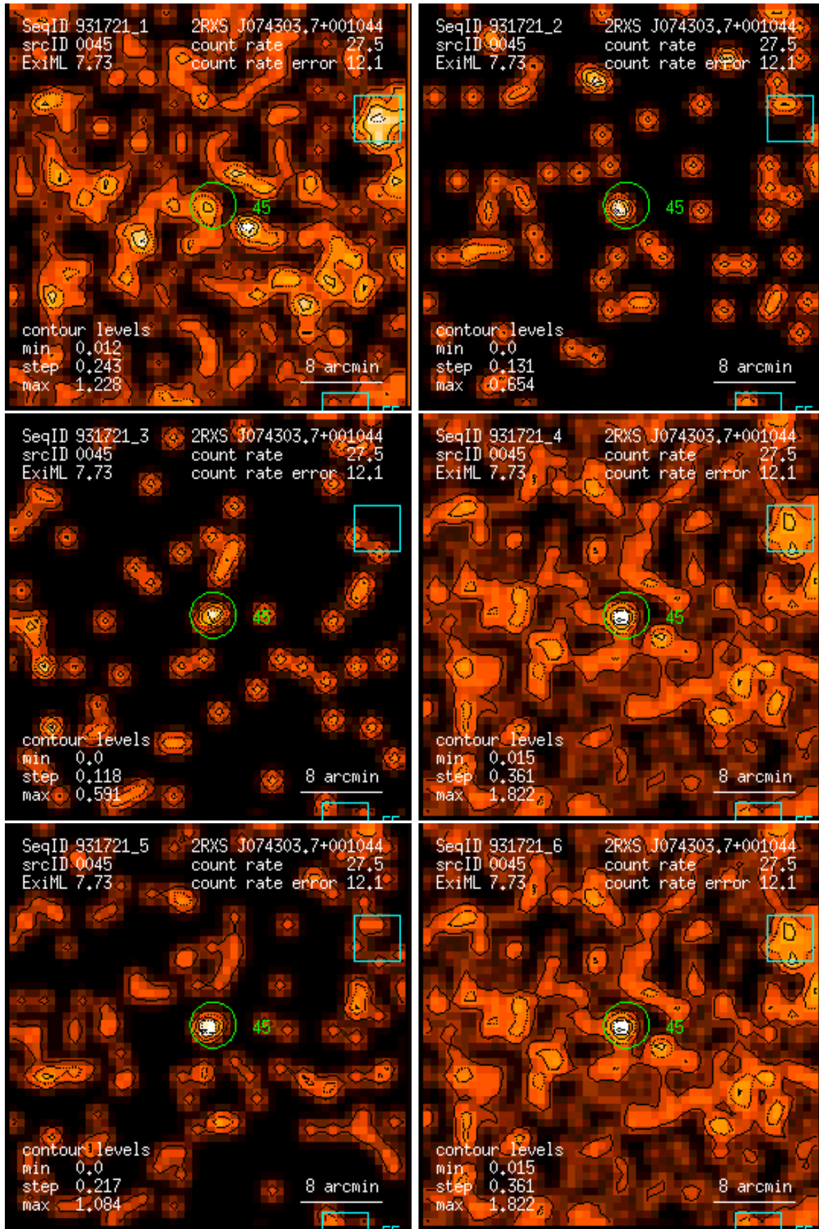
Figure 45: RASS 931721: detection 0045: band rate images, Gaussian filter: (1) PSPC channels 11 – 41, (2) 52 – 90, (3) 91 – 201, (4) 11 – 235, (5) 52 – 201, (6) 11 – 201. Broad band rates in counts/ks. Band rate contour levels in counts/ks/arcmin 2 .
