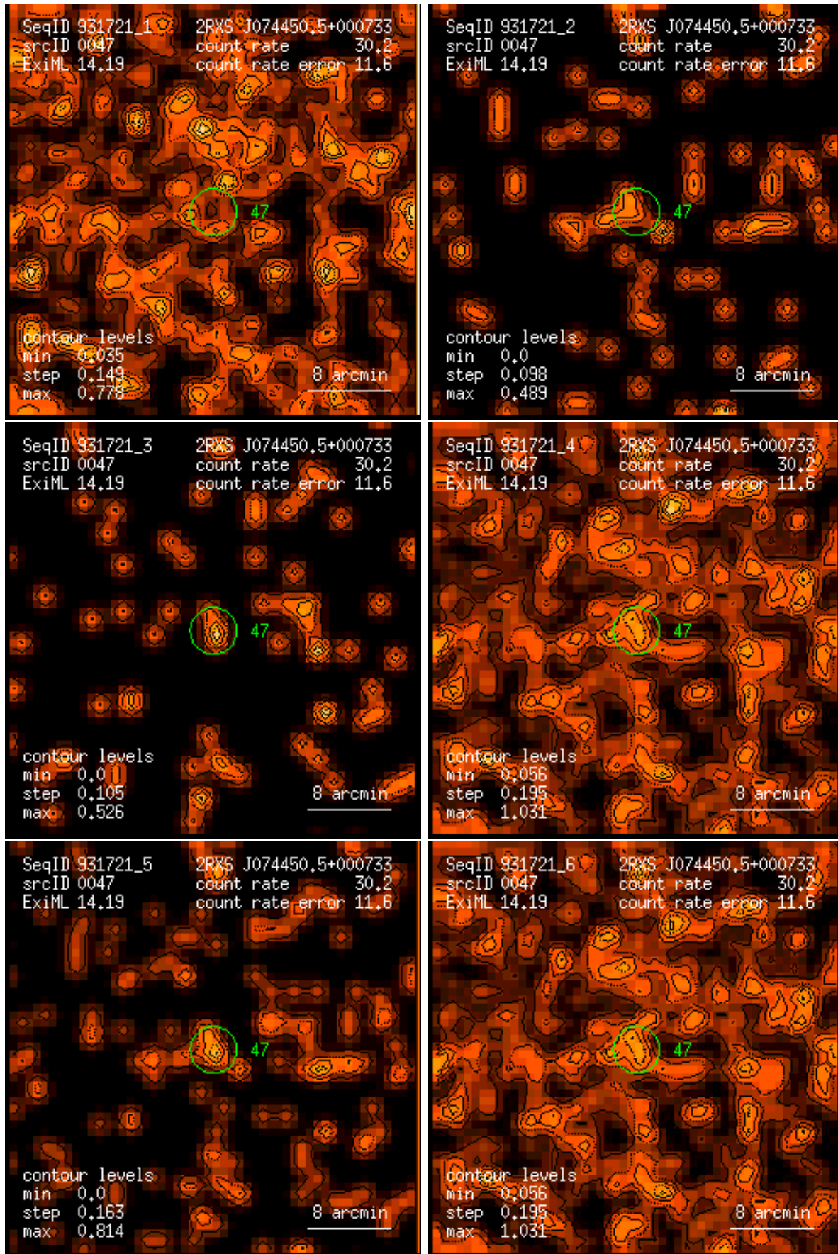
Figure 47: RASS 931721: detection 0047: band rate images, Gaussian filter: (1) PSPC channels 11 – 41, (2) 52 – 90, (3) 91 – 201, (4) 11 – 235, (5) 52 – 201, (6) 11 – 201. Broad band rates in counts/ks. Band rate contour levels in counts/ks/arcmin 2 .
