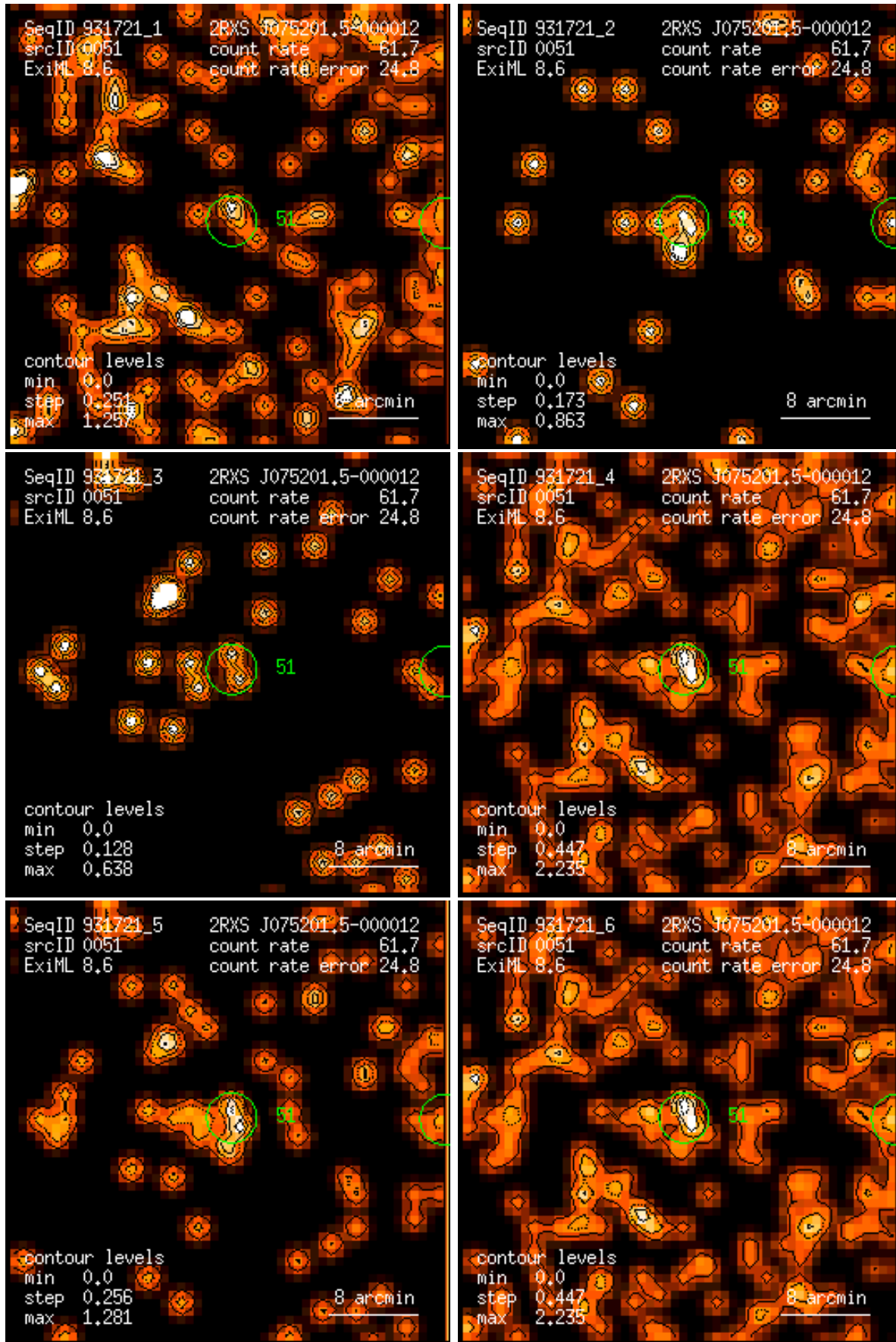
Figure 51: RASS 931721: detection 0051: band rate images, Gaussian filter: (1) PSPC channels 11 – 41, (2) 52 – 90, (3) 91 – 201, (4) 11 – 235, (5) 52 – 201, (6) 11 – 201. Broad band rates in counts/ks. Band rate contour levels in counts/ks/arcmin 2 .
