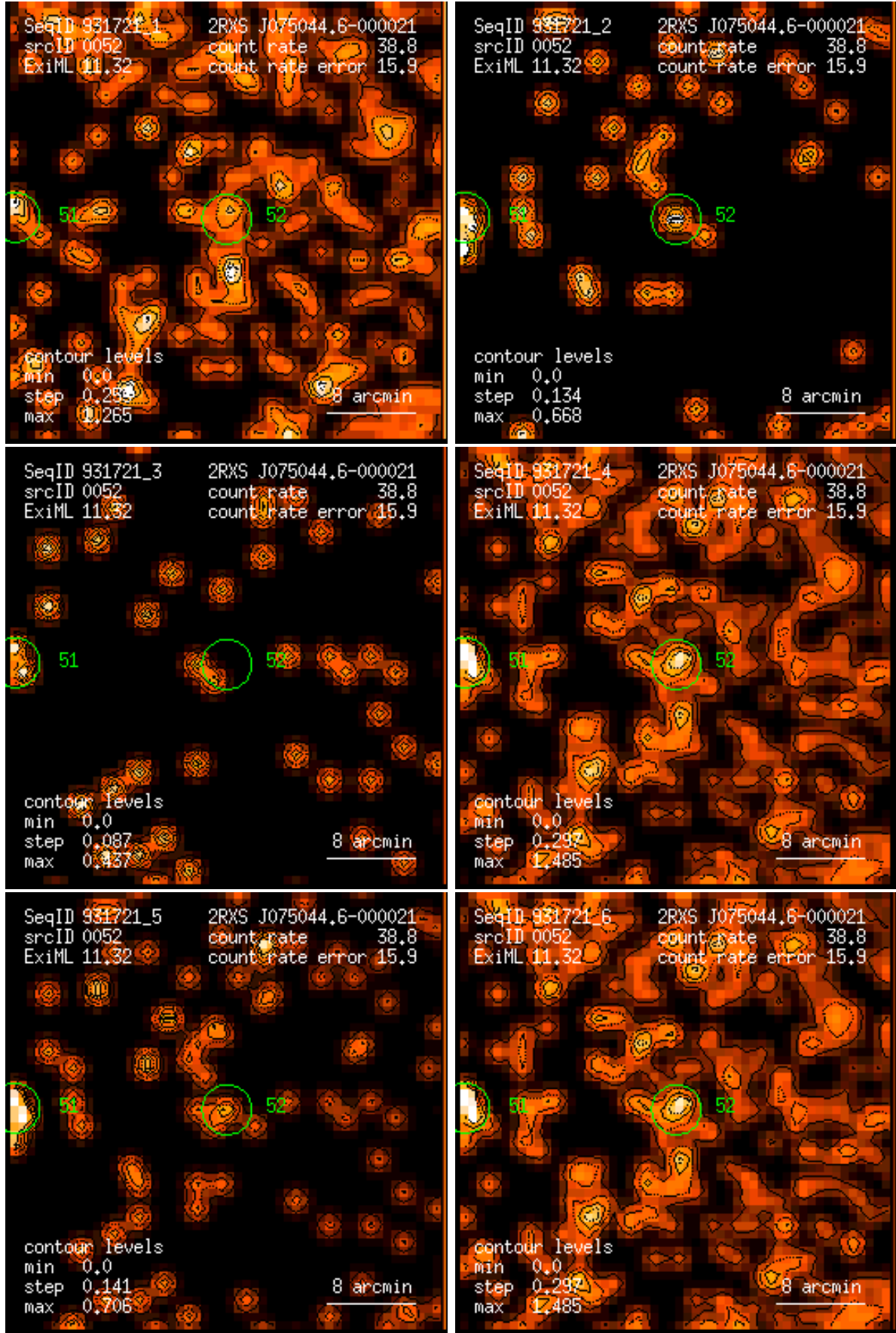
Figure 52: RASS 931721: detection 0052: band rate images, Gaussian filter: (1) PSPC channels 11 – 41, (2) 52 – 90, (3) 91 – 201, (4) 11 – 235, (5) 52 – 201, (6) 11 – 201. Broad band rates in counts/ks. Band rate contour levels in counts/ks/arcmin 2 .
