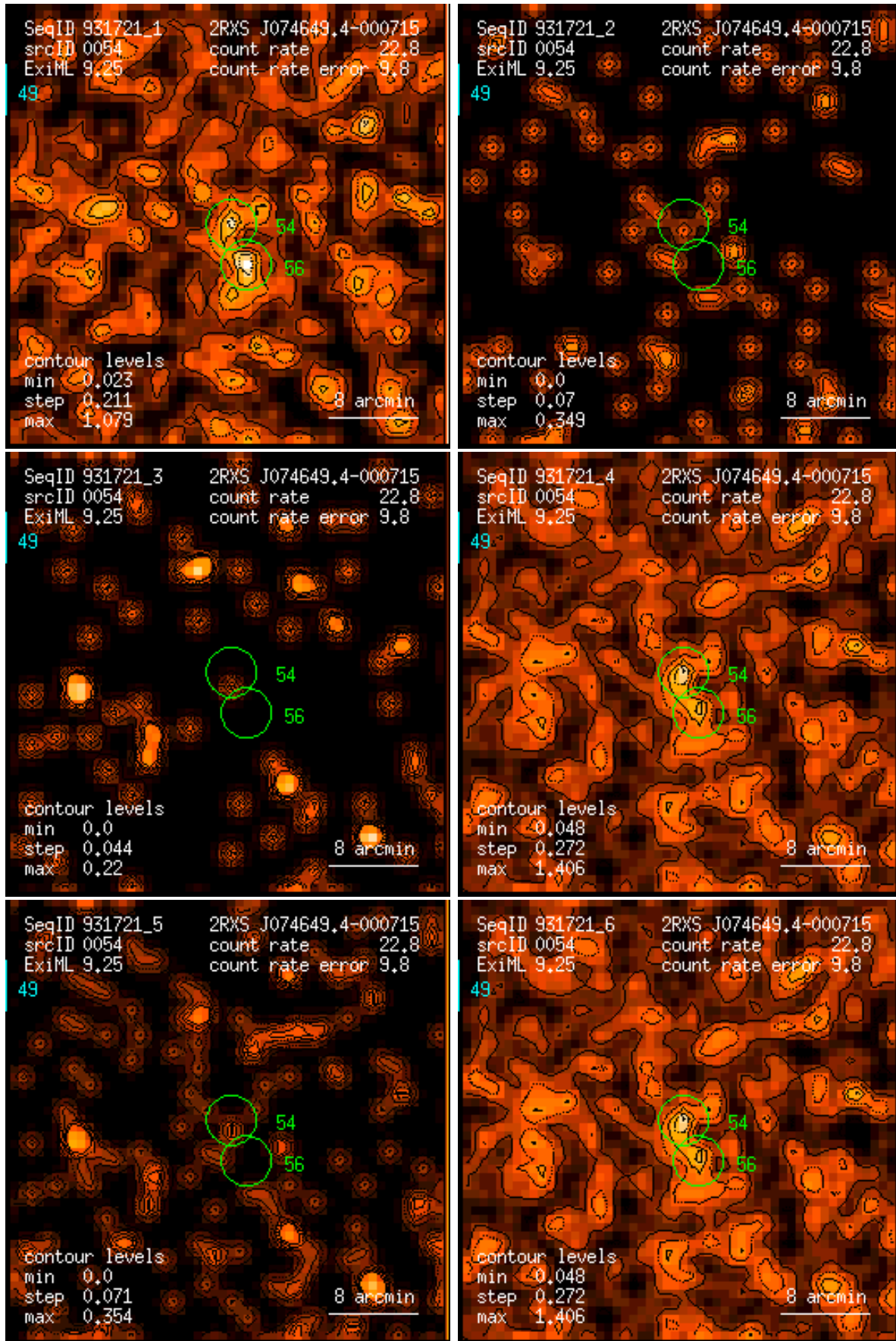
Figure 54: RASS 931721: detection 0054: band rate images, Gaussian filter: (1) PSPC channels 11 – 41, (2) 52 – 90, (3) 91 – 201, (4) 11 – 235, (5) 52 – 201, (6) 11 – 201. Broad band rates in counts/ks. Band rate contour levels in counts/ks/arcmin 2 .
