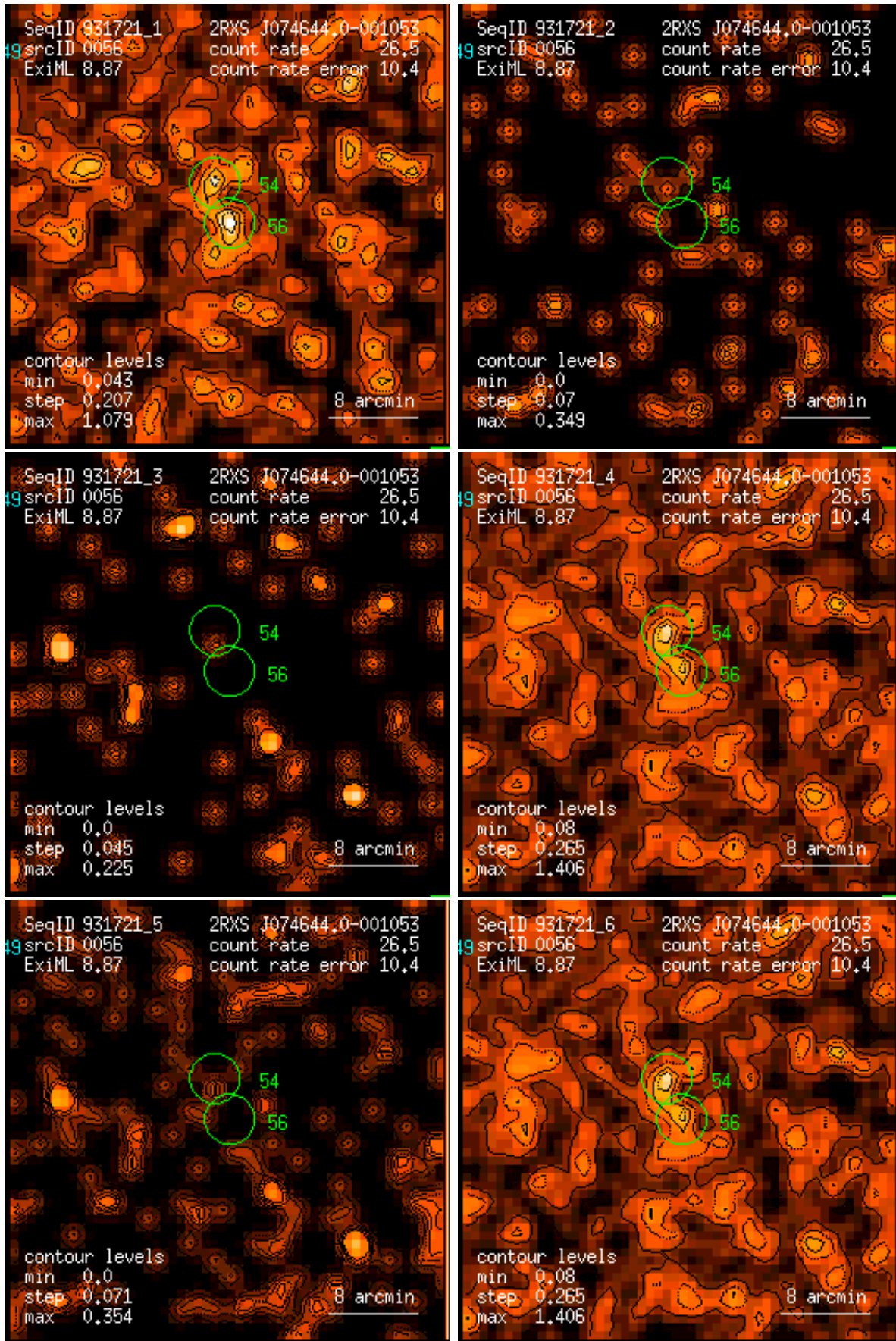
Figure 56: RASS 931721: detection 0056: band rate images, Gaussian filter: (1) PSPC channels 11 – 41, (2) 52 – 90, (3) 91 – 201, (4) 11 – 235, (5) 52 – 201, (6) 11 – 201. Broad band rates in counts/ks. Band rate contour levels in counts/ks/arcmin 2 .
