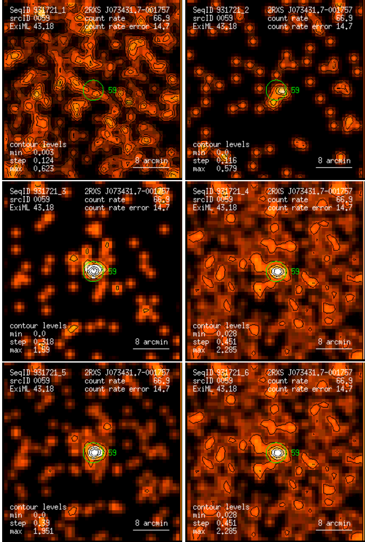
Figure 59: RASS 931721: detection 0059: band rate images, Gaussian filter: (1) PSPC channels 11 – 41, (2) 52 – 90, (3) 91 – 201, (4) 11 – 235, (5) 52 – 201, (6) 11 – 201. Broad band rates in counts/ks. Band rate contour levels in counts/ks/arcmin 2 .
