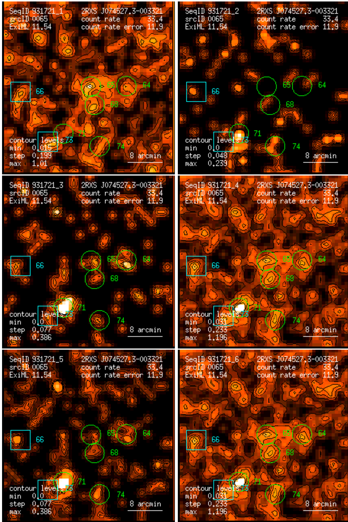
Figure 65: RASS 931721: detection 0065: band rate images, Gaussian filter: (1) PSPC channels 11 – 41, (2) 52 – 90, (3) 91 – 201, (4) 11 – 235, (5) 52 – 201, (6) 11 – 201. Broad band rates in counts/ks. Band rate contour levels in counts/ks/arcmin 2 .
