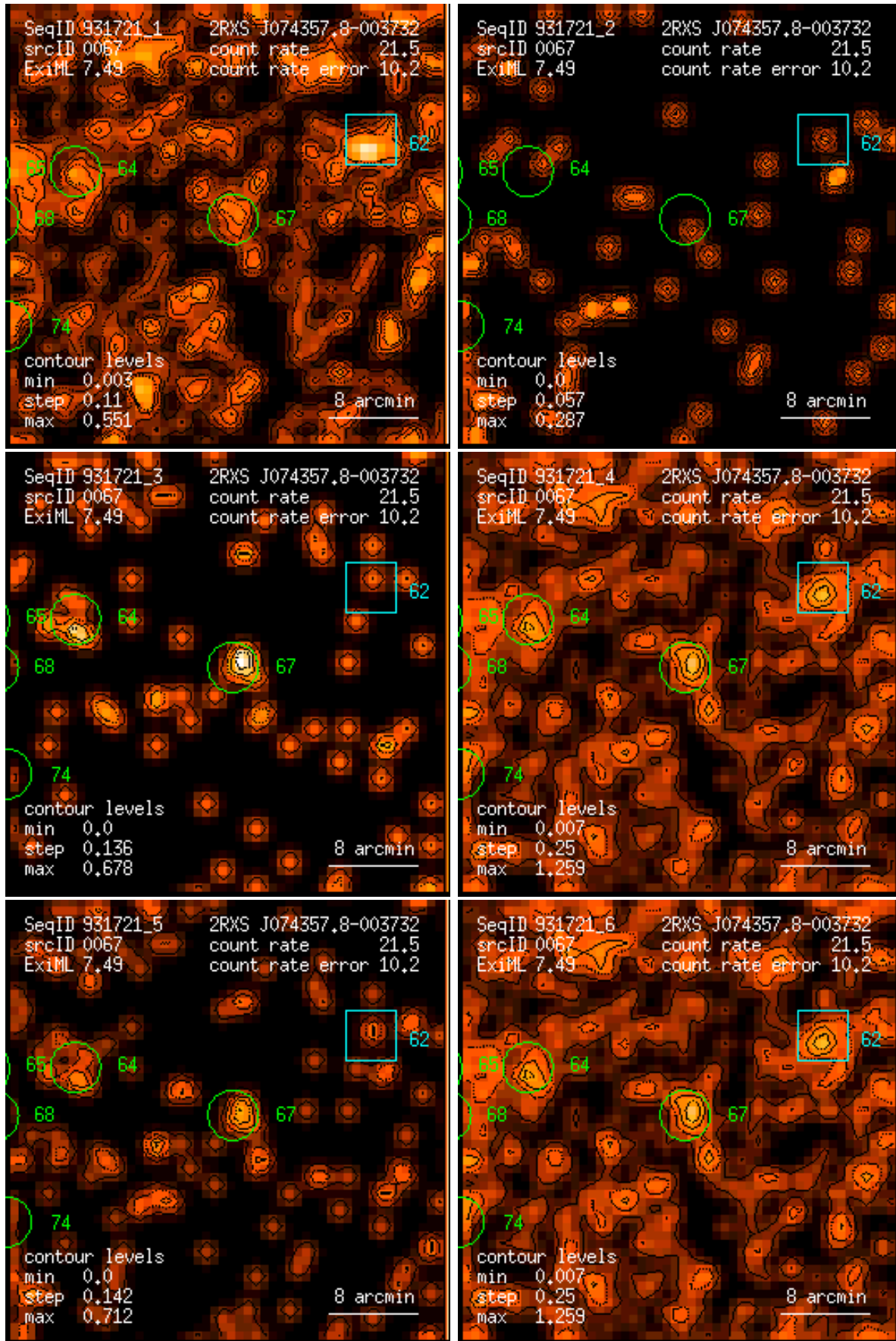
Figure 67: RASS 931721: detection 0067: band rate images, Gaussian filter: (1) PSPC channels 11 – 41, (2) 52 – 90, (3) 91 – 201, (4) 11 – 235, (5) 52 – 201, (6) 11 – 201. Broad band rates in counts/ks. Band rate contour levels in counts/ks/arcmin 2 .
