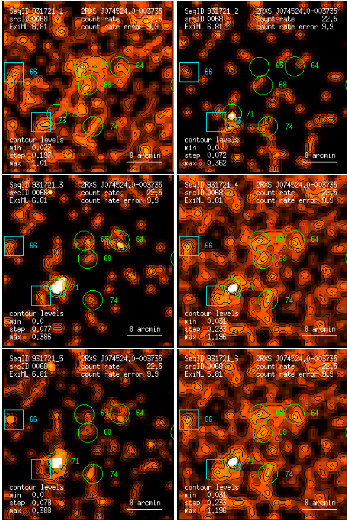
Figure 68: RASS 931721: detection 0068: band rate images, Gaussian filter: (1) PSPC channels 11 – 41, (2) 52 – 90, (3) 91 – 201, (4) 11 – 235, (5) 52 – 201, (6) 11 – 201. Broad band rates in counts/ks. Band rate contour levels in counts/ks/arcmin 2 .
