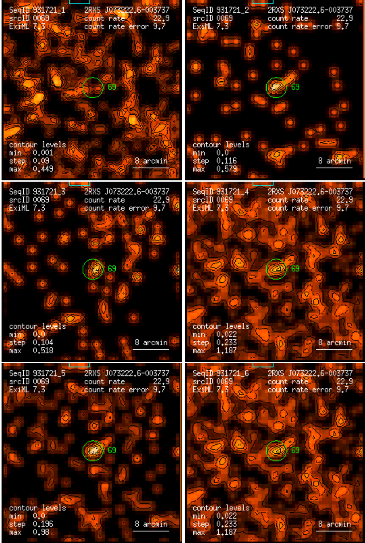
Figure 69: RASS 931721: detection 0069: band rate images, Gaussian filter: (1) PSPC channels 11 – 41, (2) 52 – 90, (3) 91 – 201, (4) 11 – 235, (5) 52 – 201, (6) 11 – 201. Broad band rates in counts/ks. Band rate contour levels in counts/ks/arcmin 2 .
