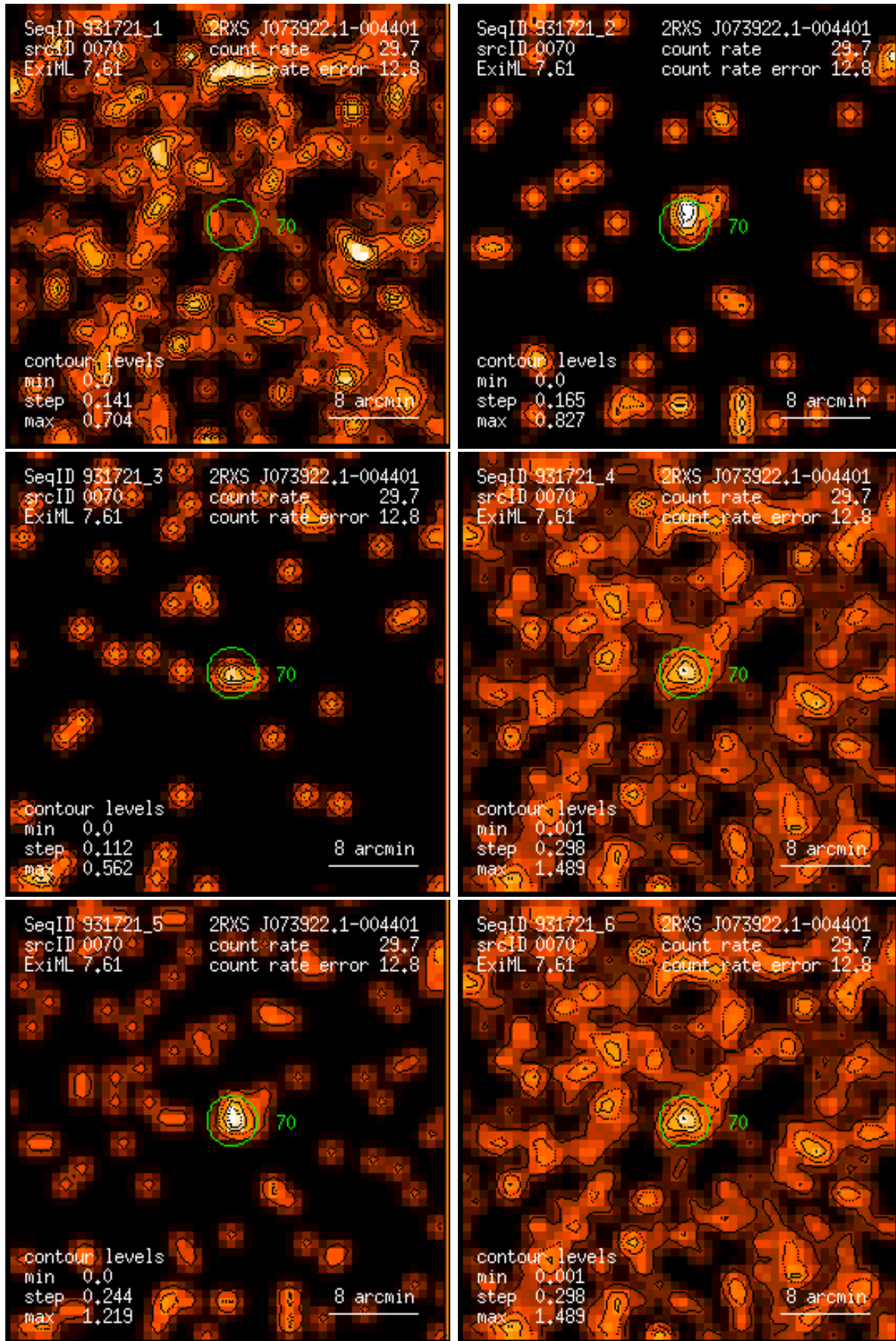
Figure 70: RASS 931721: detection 0070: band rate images, Gaussian filter: (1) PSPC channels 11 – 41, (2) 52 – 90, (3) 91 – 201, (4) 11 – 235, (5) 52 – 201, (6) 11 – 201. Broad band rates in counts/ks. Band rate contour levels in counts/ks/arcmin 2 .
