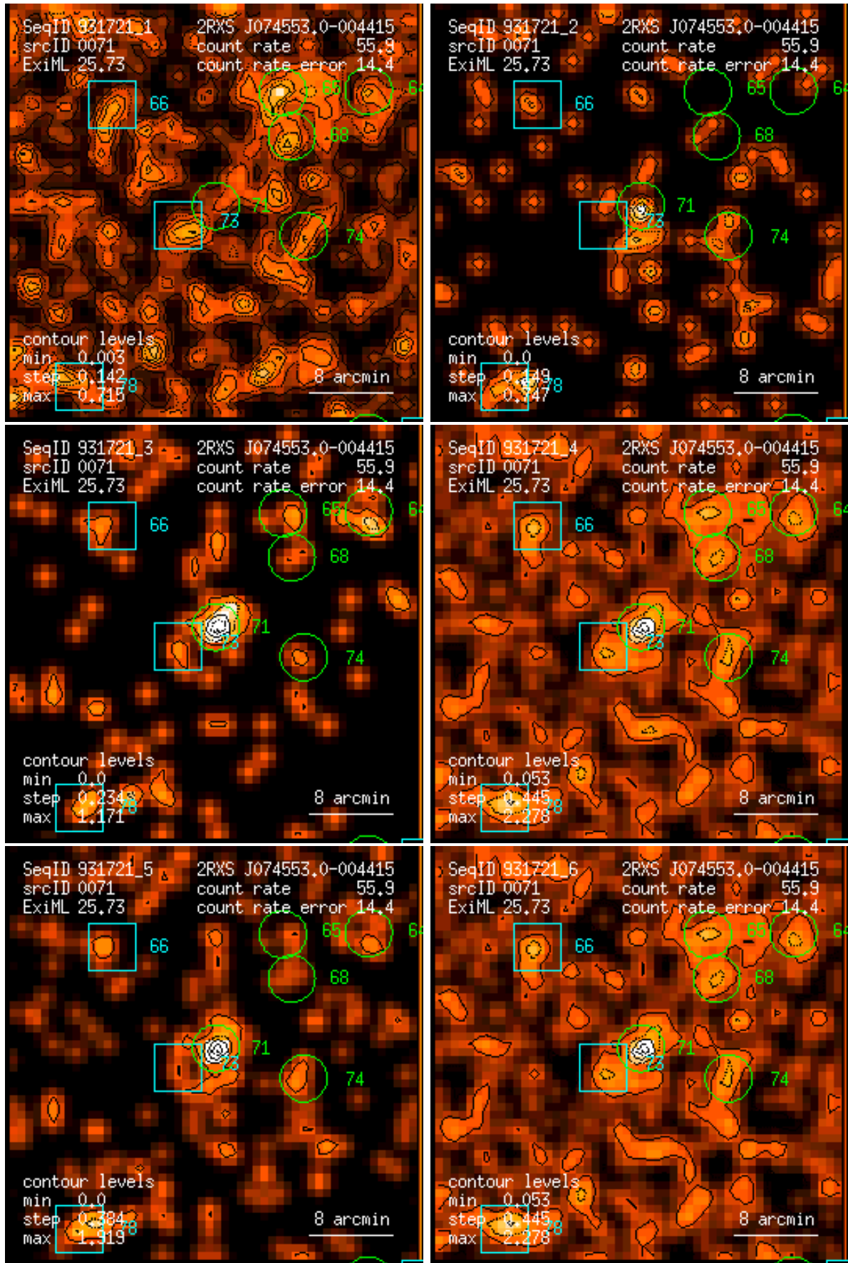
Figure 71: RASS 931721: detection 0071: band rate images, Gaussian filter: (1) PSPC channels 11 – 41, (2) 52 – 90, (3) 91 – 201, (4) 11 – 235, (5) 52 – 201, (6) 11 – 201. Broad band rates in counts/ks. Band rate contour levels in counts/ks/arcmin 2 .
