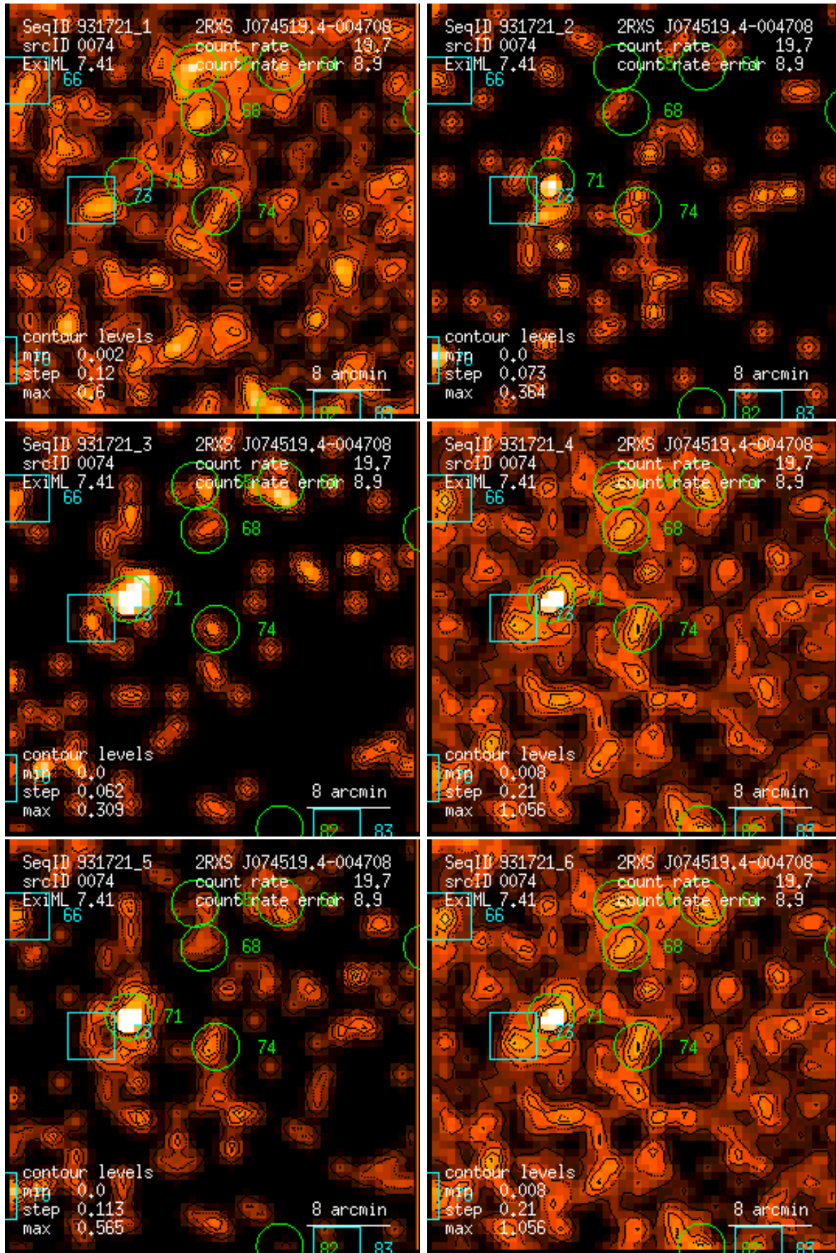
Figure 74: RASS 931721: detection 0074: band rate images, Gaussian filter: (1) PSPC channels 11 – 41, (2) 52 – 90, (3) 91 – 201, (4) 11 – 235, (5) 52 – 201, (6) 11 – 201. Broad band rates in counts/ks. Band rate contour levels in counts/ks/arcmin 2 .
