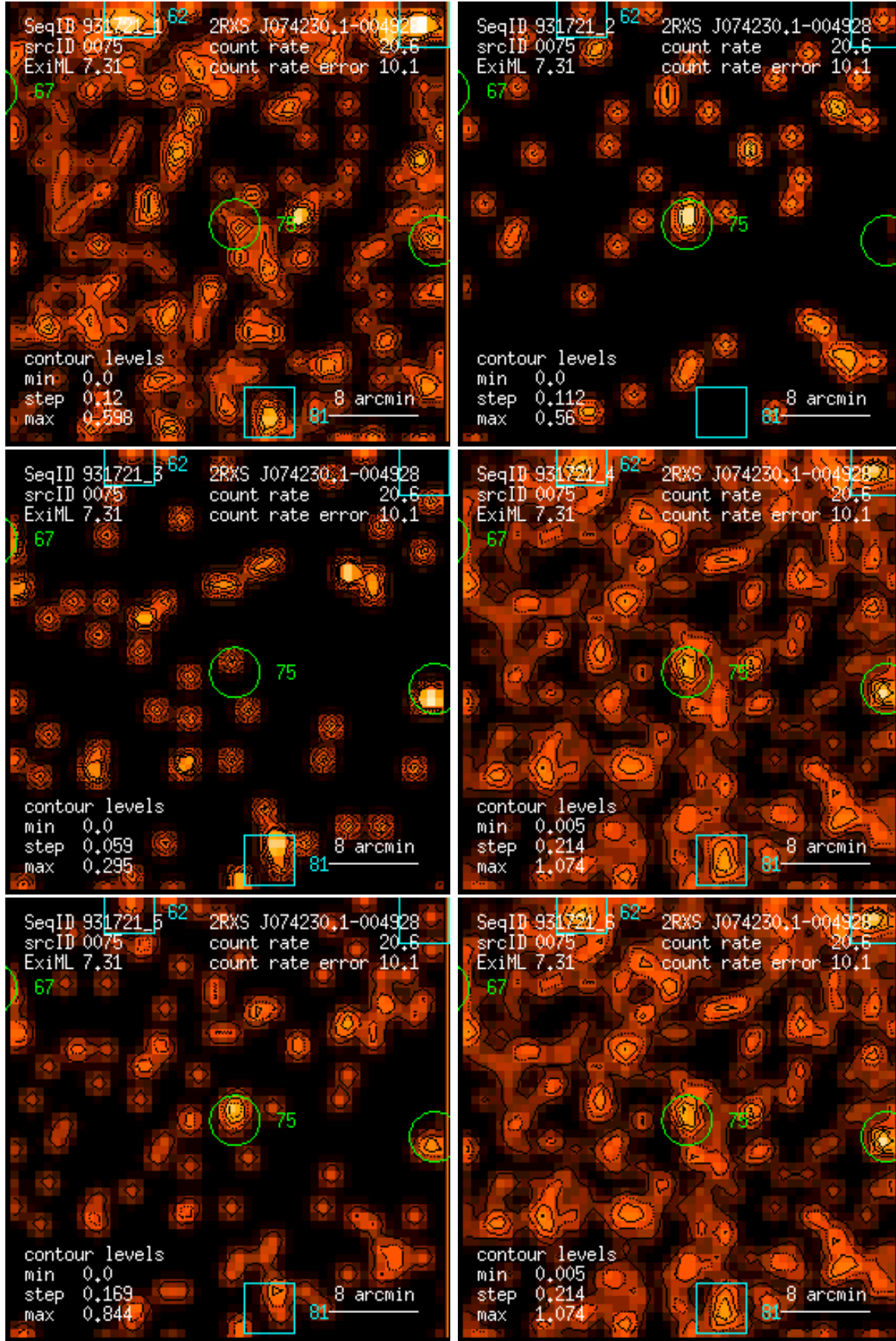
Figure 75: RASS 931721: detection 0075: band rate images, Gaussian filter: (1) PSPC channels 11 – 41, (2) 52 – 90, (3) 91 – 201, (4) 11 – 235, (5) 52 – 201, (6) 11 – 201. Broad band rates in counts/ks. Band rate contour levels in counts/ks/arcmin 2 .
