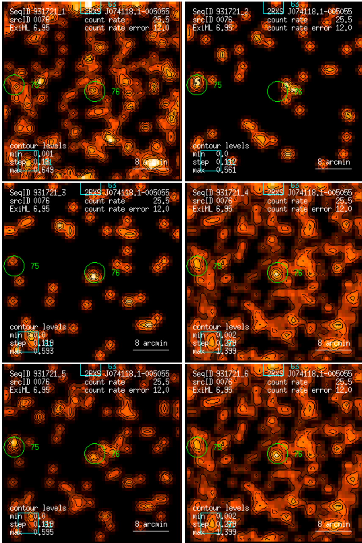
Figure 76: RASS 931721: detection 0076: band rate images, Gaussian filter: (1) PSPC channels 11 – 41, (2) 52 – 90, (3) 91 – 201, (4) 11 – 235, (5) 52 – 201, (6) 11 – 201. Broad band rates in counts/ks. Band rate contour levels in counts/ks/arcmin 2 .
