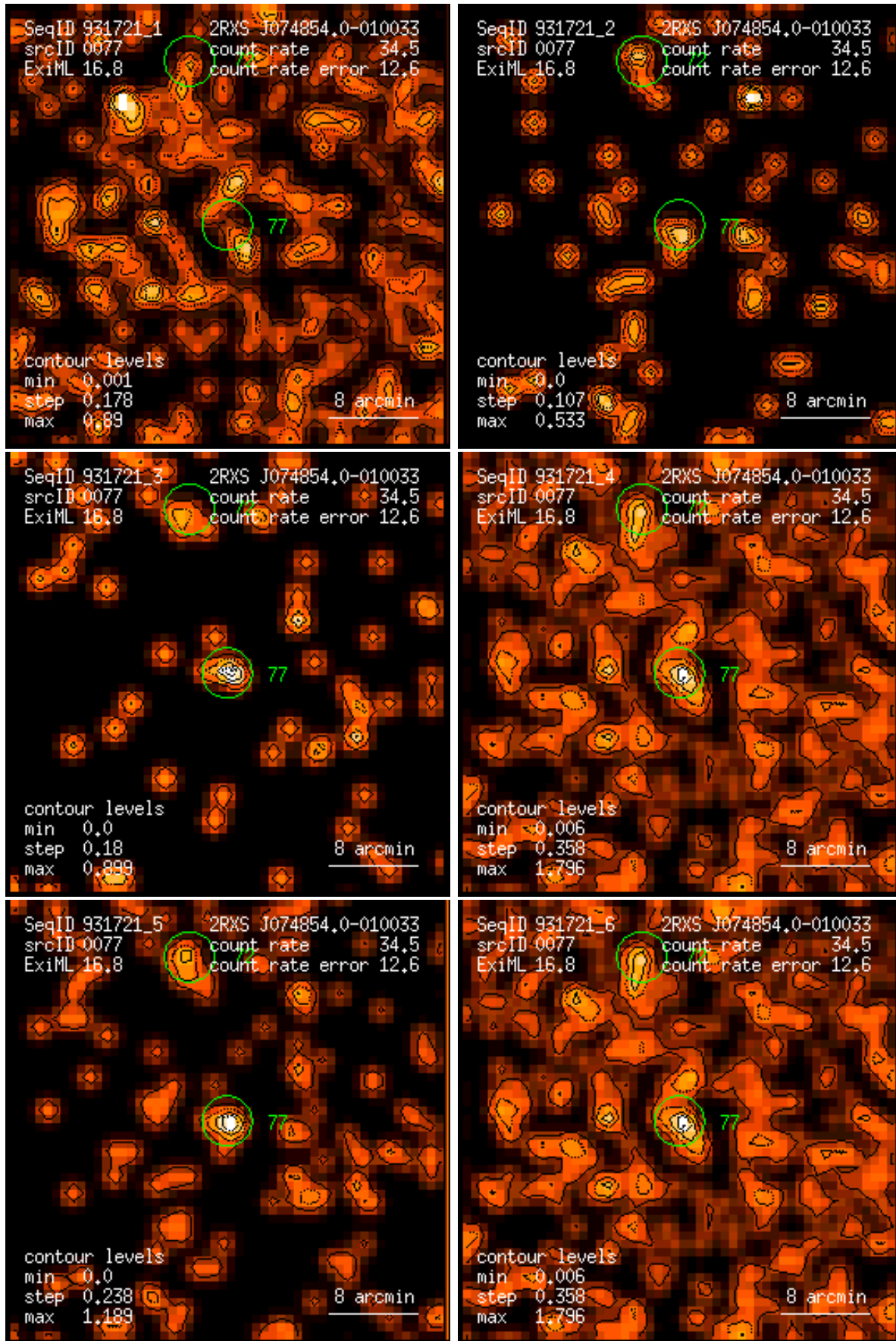
Figure 77: RASS 931721: detection 0077: band rate images, Gaussian filter: (1) PSPC channels 11 – 41, (2) 52 – 90, (3) 91 – 201, (4) 11 – 235, (5) 52 – 201, (6) 11 – 201. Broad band rates in counts/ks. Band rate contour levels in counts/ks/arcmin 2 .
