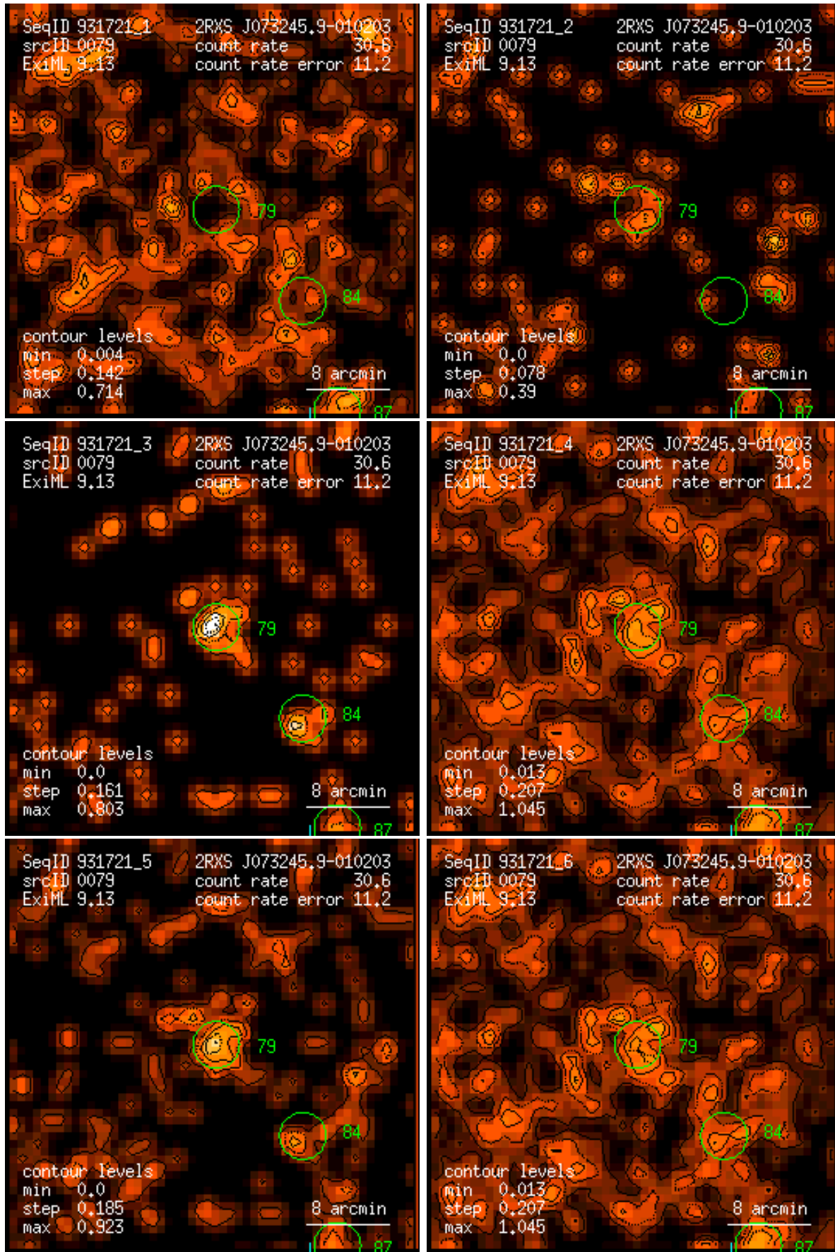
Figure 79: RASS 931721: detection 0079: band rate images, Gaussian filter: (1) PSPC channels 11 – 41, (2) 52 – 90, (3) 91 – 201, (4) 11 – 235, (5) 52 – 201, (6) 11 – 201. Broad band rates in counts/ks. Band rate contour levels in counts/ks/arcmin 2 .
