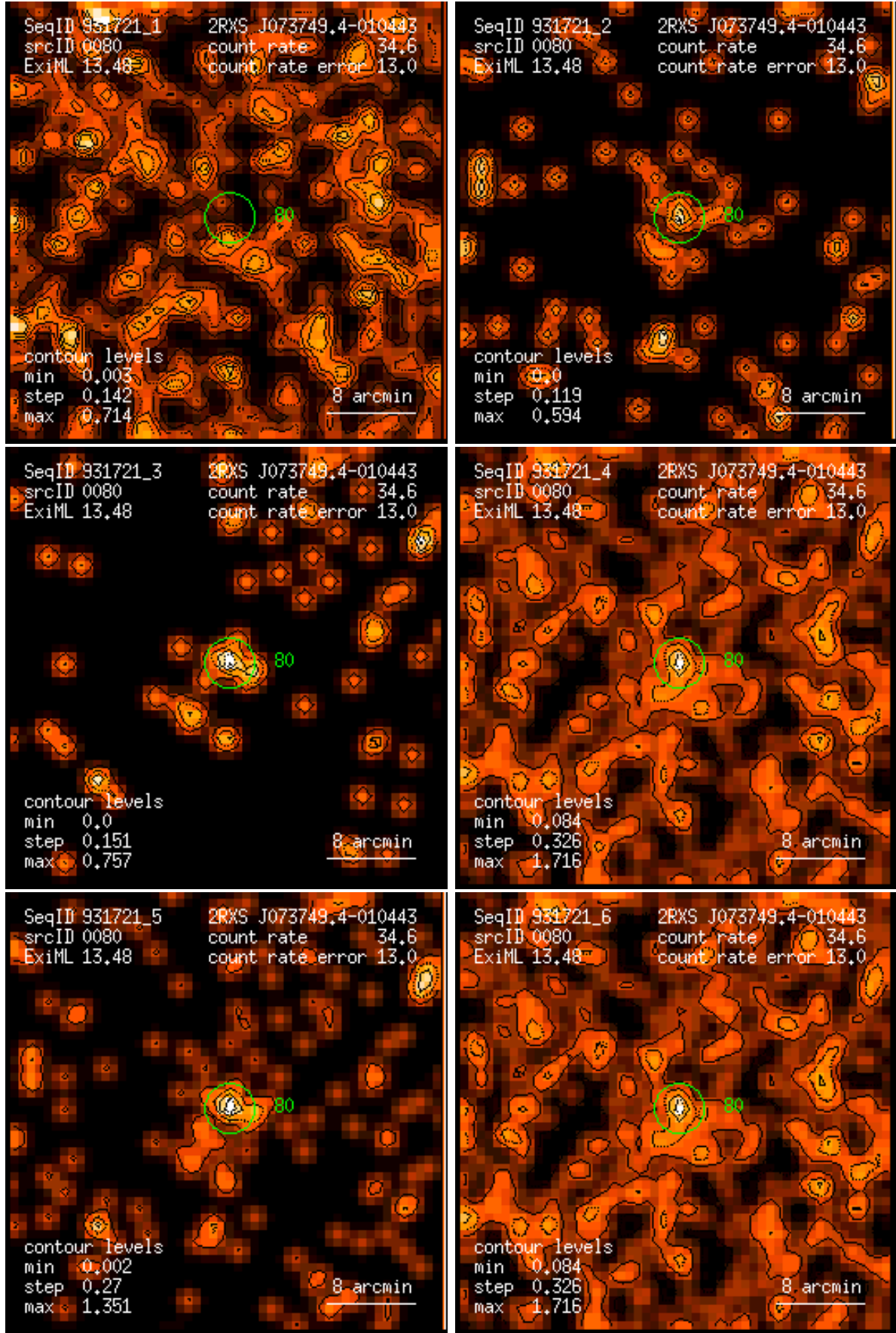
Figure 80: RASS 931721: detection 0080: band rate images, Gaussian filter: (1) PSPC channels 11 – 41, (2) 52 – 90, (3) 91 – 201, (4) 11 – 235, (5) 52 – 201, (6) 11 – 201. Broad band rates in counts/ks. Band rate contour levels in counts/ks/arcmin 2 .
