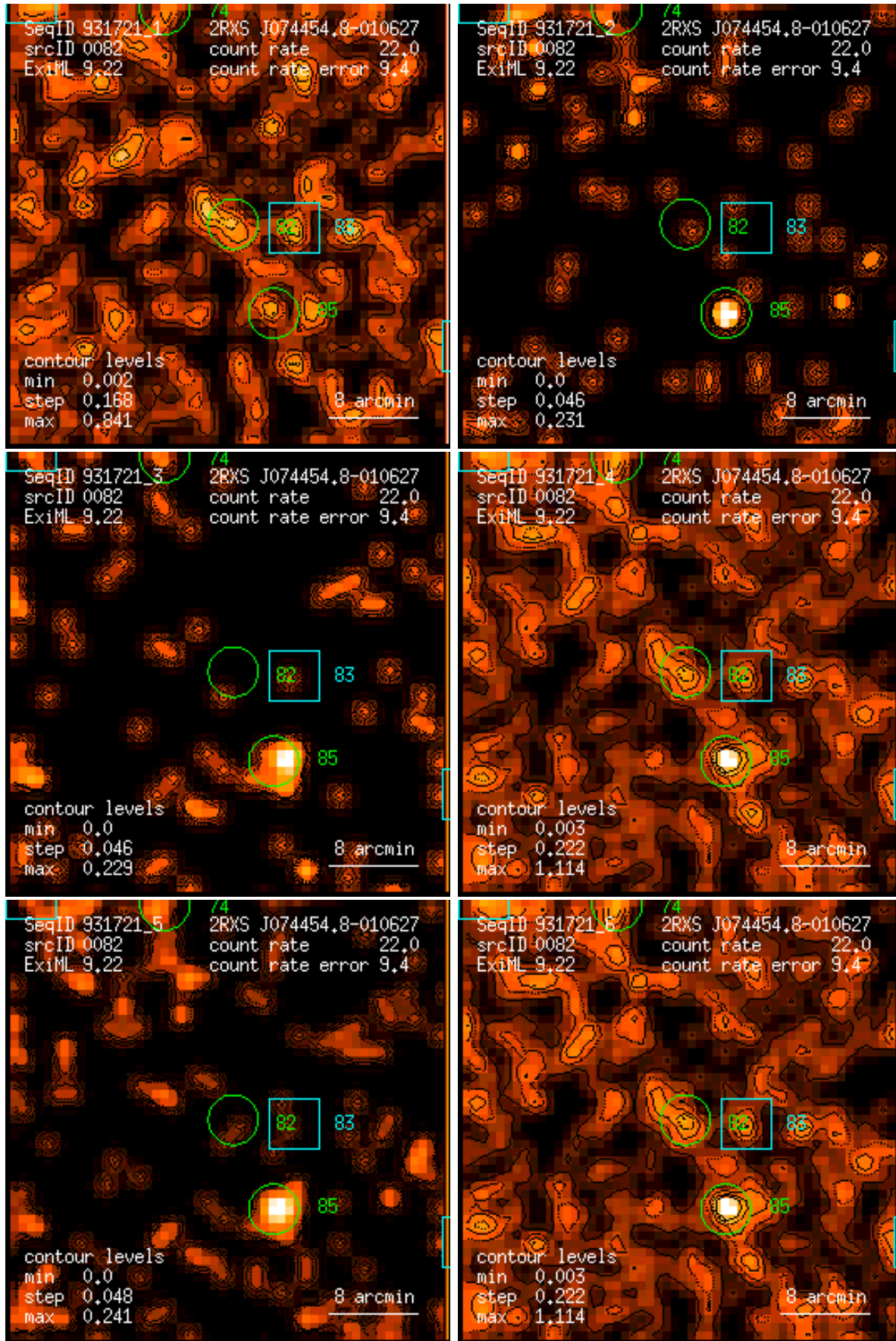
Figure 82: RASS 931721: detection 0082: band rate images, Gaussian filter: (1) PSPC channels 11 – 41, (2) 52 – 90, (3) 91 – 201, (4) 11 – 235, (5) 52 – 201, (6) 11 – 201. Broad band rates in counts/ks. Band rate contour levels in counts/ks/arcmin 2 .
