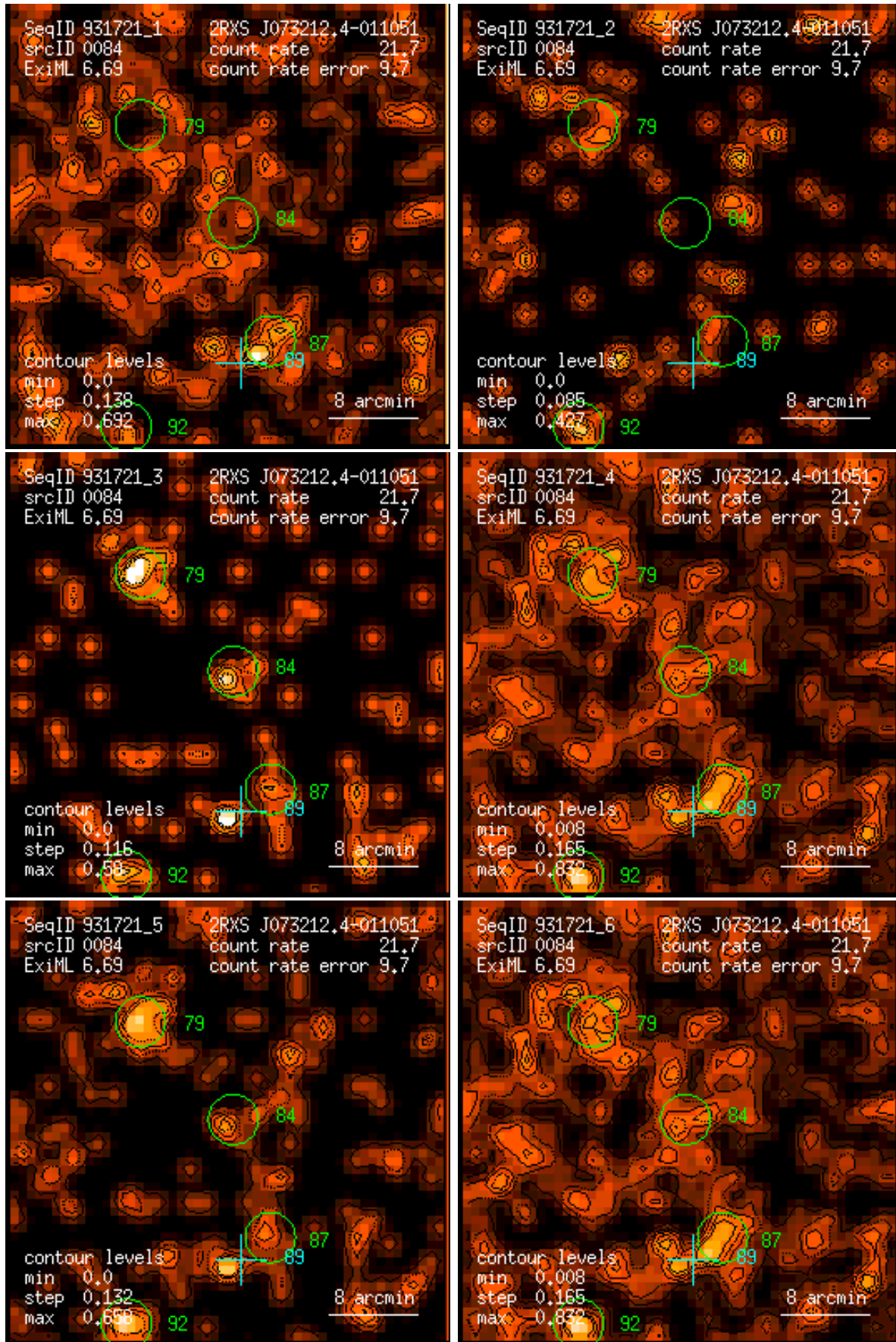
Figure 84: RASS 931721: detection 0084: band rate images, Gaussian filter: (1) PSPC channels 11 – 41, (2) 52 – 90, (3) 91 – 201, (4) 11 – 235, (5) 52 – 201, (6) 11 – 201. Broad band rates in counts/ks. Band rate contour levels in counts/ks/arcmin 2 .
