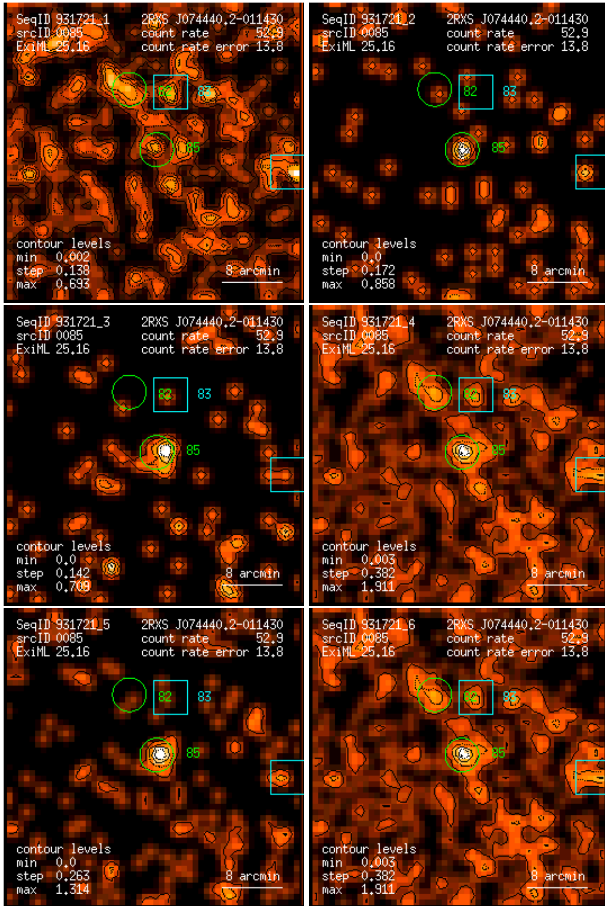
Figure 85: RASS 931721: detection 0085: band rate images, Gaussian filter: (1) PSPC channels 11 – 41, (2) 52 – 90, (3) 91 – 201, (4) 11 – 235, (5) 52 – 201, (6) 11 – 201. Broad band rates in counts/ks. Band rate contour levels in counts/ks/arcmin 2 .
