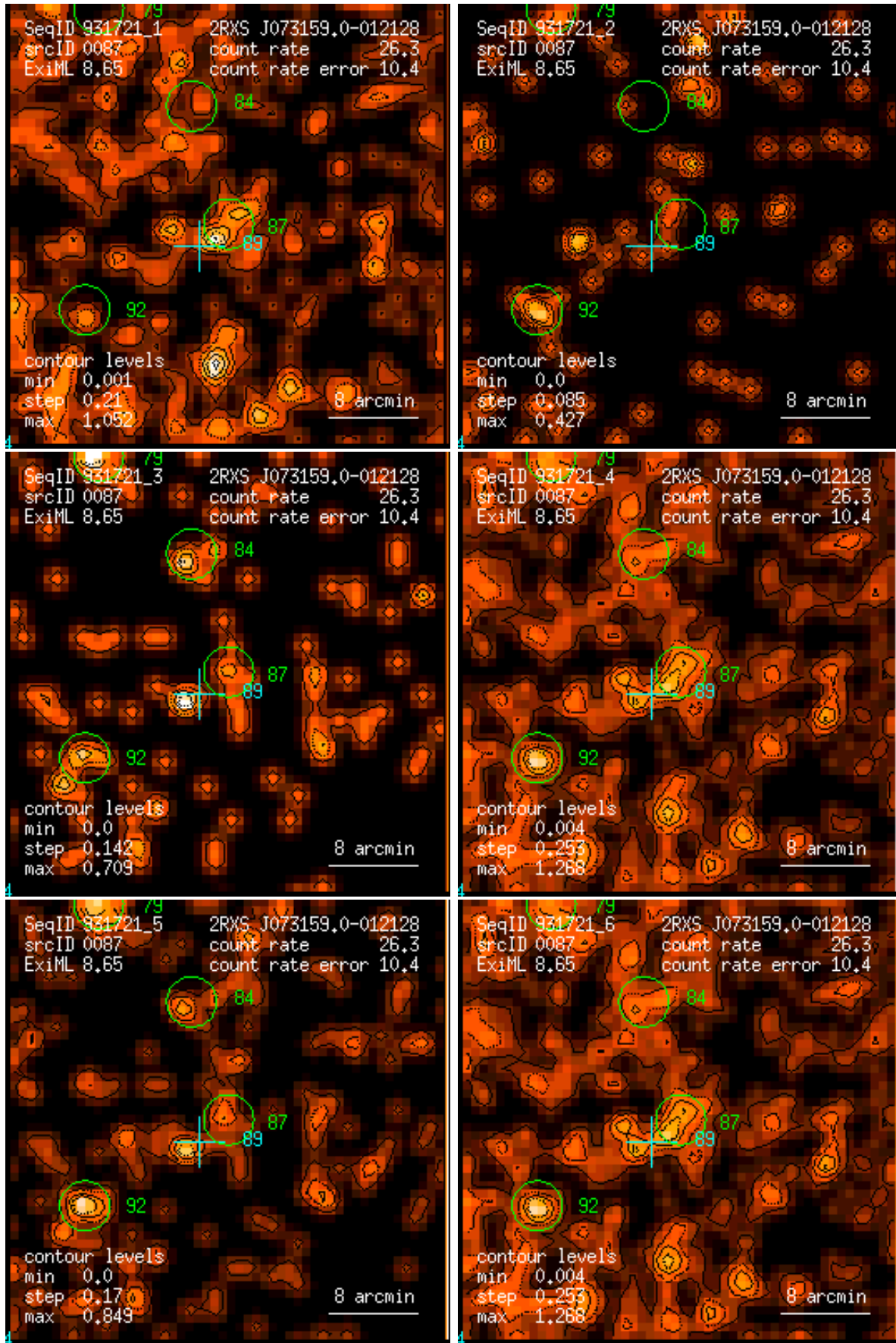
Figure 87: RASS 931721: detection 0087: band rate images, Gaussian filter: (1) PSPC channels 11 – 41, (2) 52 – 90, (3) 91 – 201, (4) 11 – 235, (5) 52 – 201, (6) 11 – 201. Broad band rates in counts/ks. Band rate contour levels in counts/ks/arcmin 2 .
