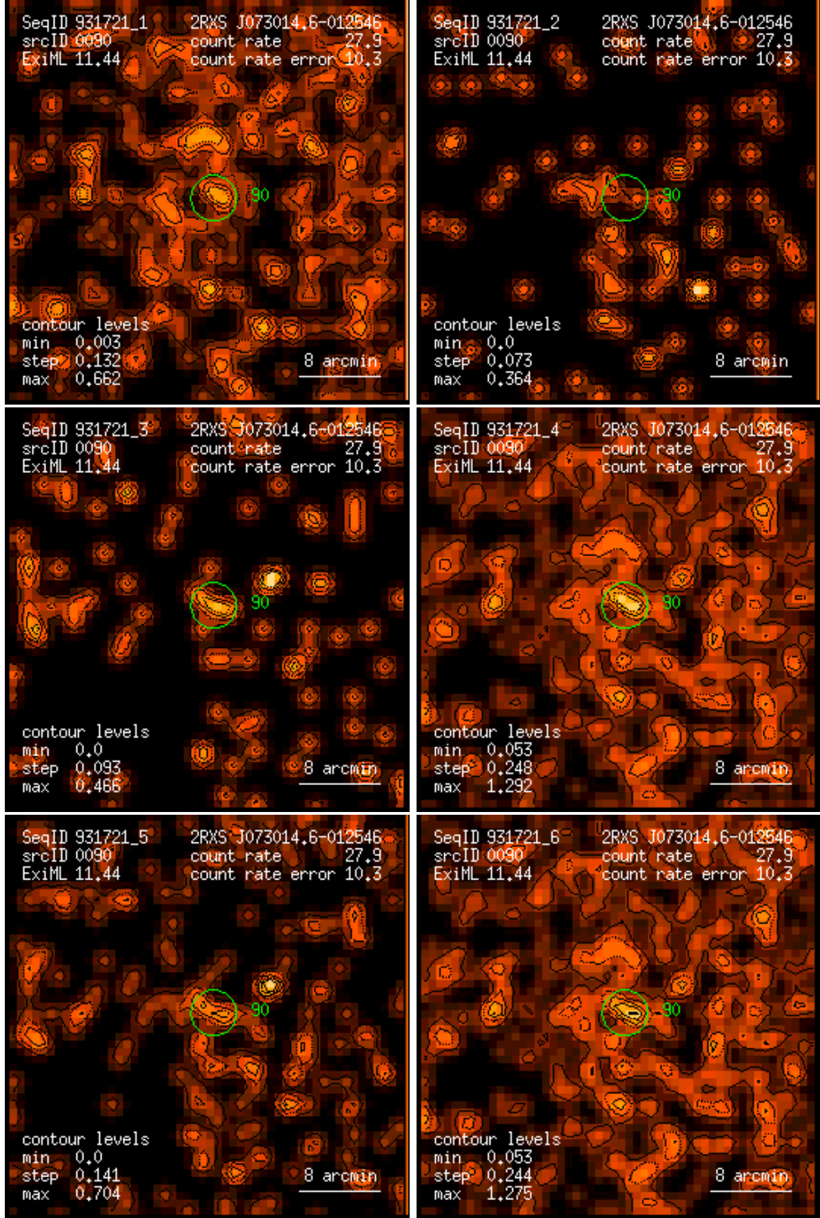
Figure 90: RASS 931721: detection 0090: band rate images, Gaussian filter: (1) PSPC channels 11 – 41, (2) 52 – 90, (3) 91 – 201, (4) 11 – 235, (5) 52 – 201, (6) 11 – 201. Broad band rates in counts/ks. Band rate contour levels in counts/ks/arcmin 2 .
