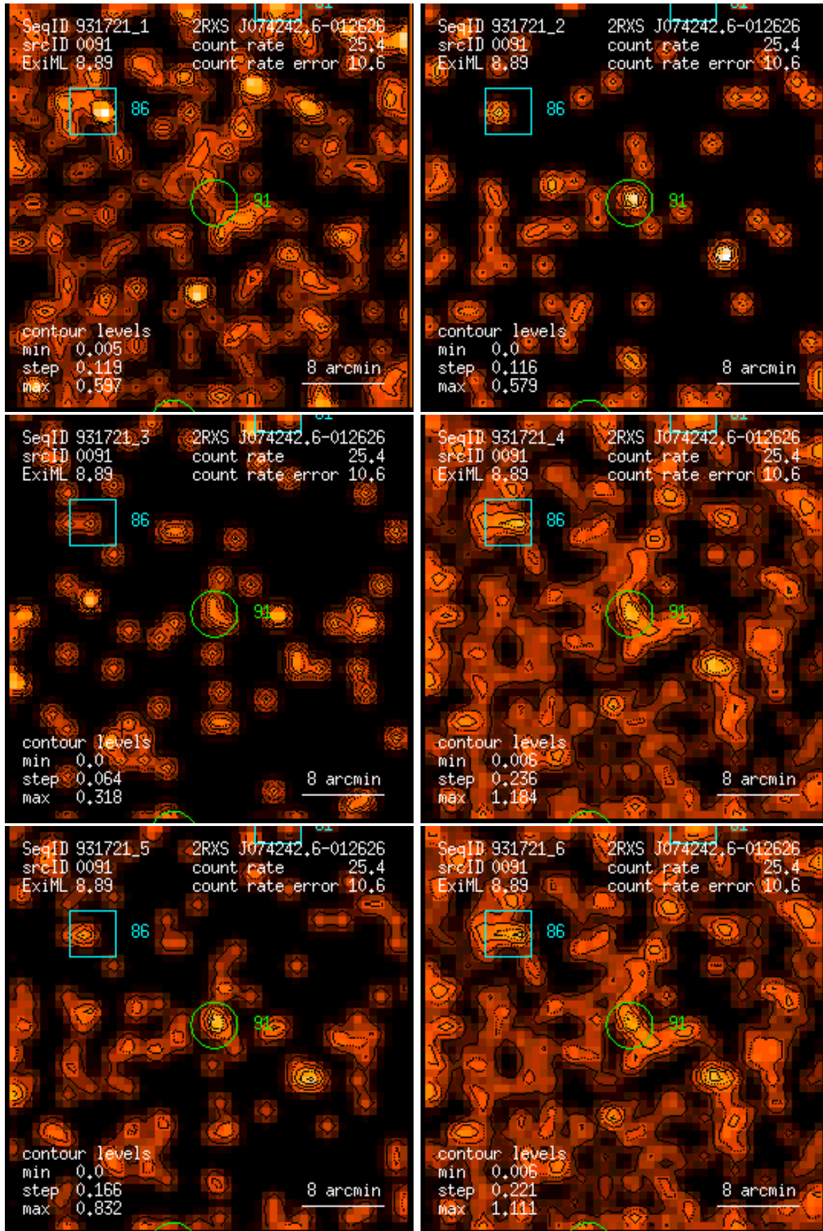
Figure 91: RASS 931721: detection 0091: band rate images, Gaussian filter: (1) PSPC channels 11 – 41, (2) 52 – 90, (3) 91 – 201, (4) 11 – 235, (5) 52 – 201, (6) 11 – 201. Broad band rates in counts/ks. Band rate contour levels in counts/ks/arcmin 2 .
