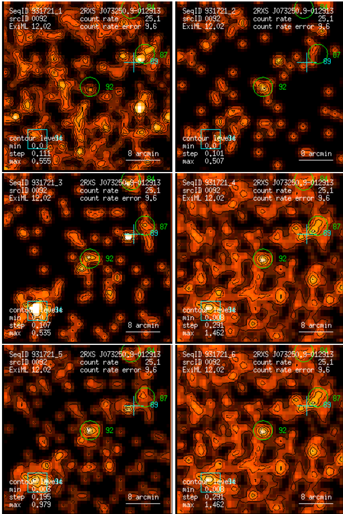
Figure 92: RASS 931721: detection 0092: band rate images, Gaussian filter: (1) PSPC channels 11 – 41, (2) 52 – 90, (3) 91 – 201, (4) 11 – 235, (5) 52 – 201, (6) 11 – 201. Broad band rates in counts/ks. Band rate contour levels in counts/ks/arcmin 2 .
