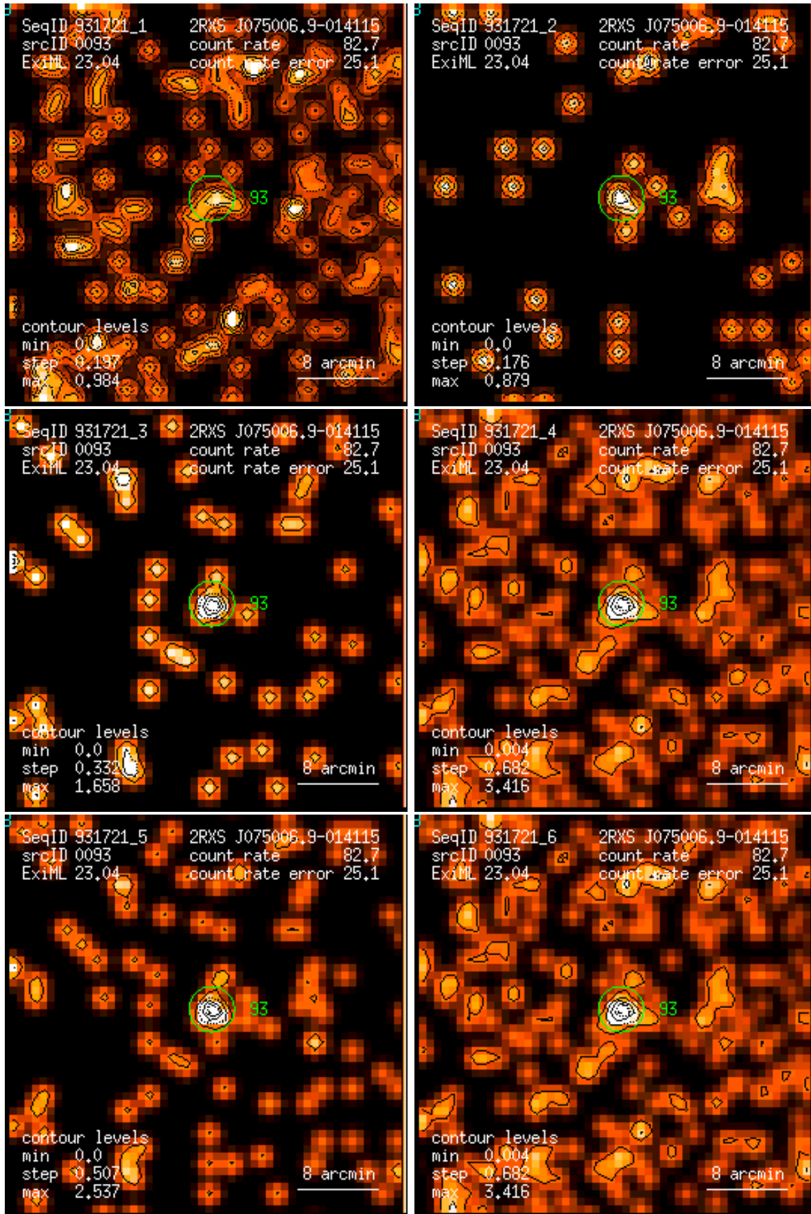
Figure 93: RASS 931721: detection 0093: band rate images, Gaussian filter: (1) PSPC channels 11 – 41, (2) 52 – 90, (3) 91 – 201, (4) 11 – 235, (5) 52 – 201, (6) 11 – 201. Broad band rates in counts/ks. Band rate contour levels in counts/ks/arcmin 2 .
