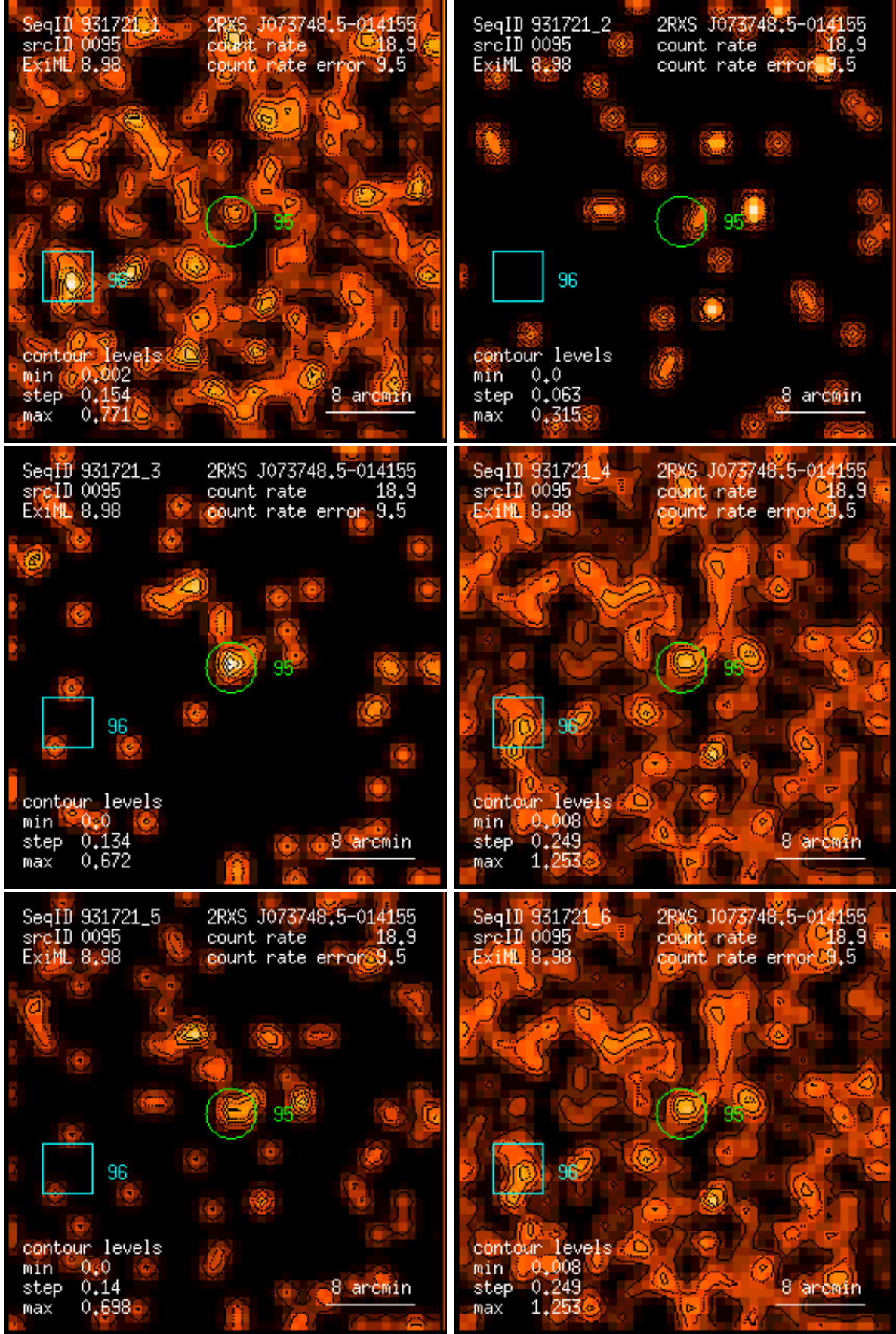
Figure 95: RASS 931721: detection 0095: band rate images, Gaussian filter: (1) PSPC channels 11 – 41, (2) 52 – 90, (3) 91 – 201, (4) 11 – 235, (5) 52 – 201, (6) 11 – 201. Broad band rates in counts/ks. Band rate contour levels in counts/ks/arcmin 2 .
