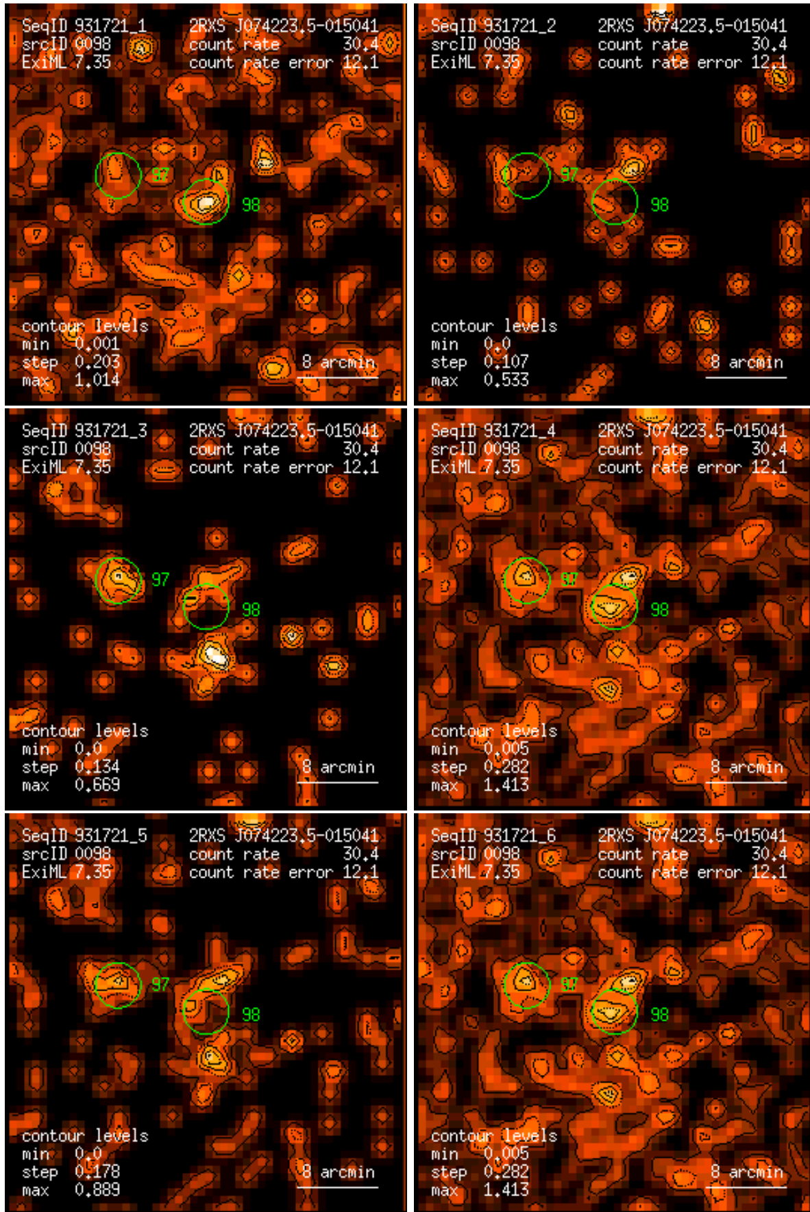
Figure 98: RASS 931721: detection 0098: band rate images, Gaussian filter: (1) PSPC channels 11 – 41, (2) 52 – 90, (3) 91 – 201, (4) 11 – 235, (5) 52 – 201, (6) 11 – 201. Broad band rates in counts/ks. Band rate contour levels in counts/ks/arcmin 2 .
