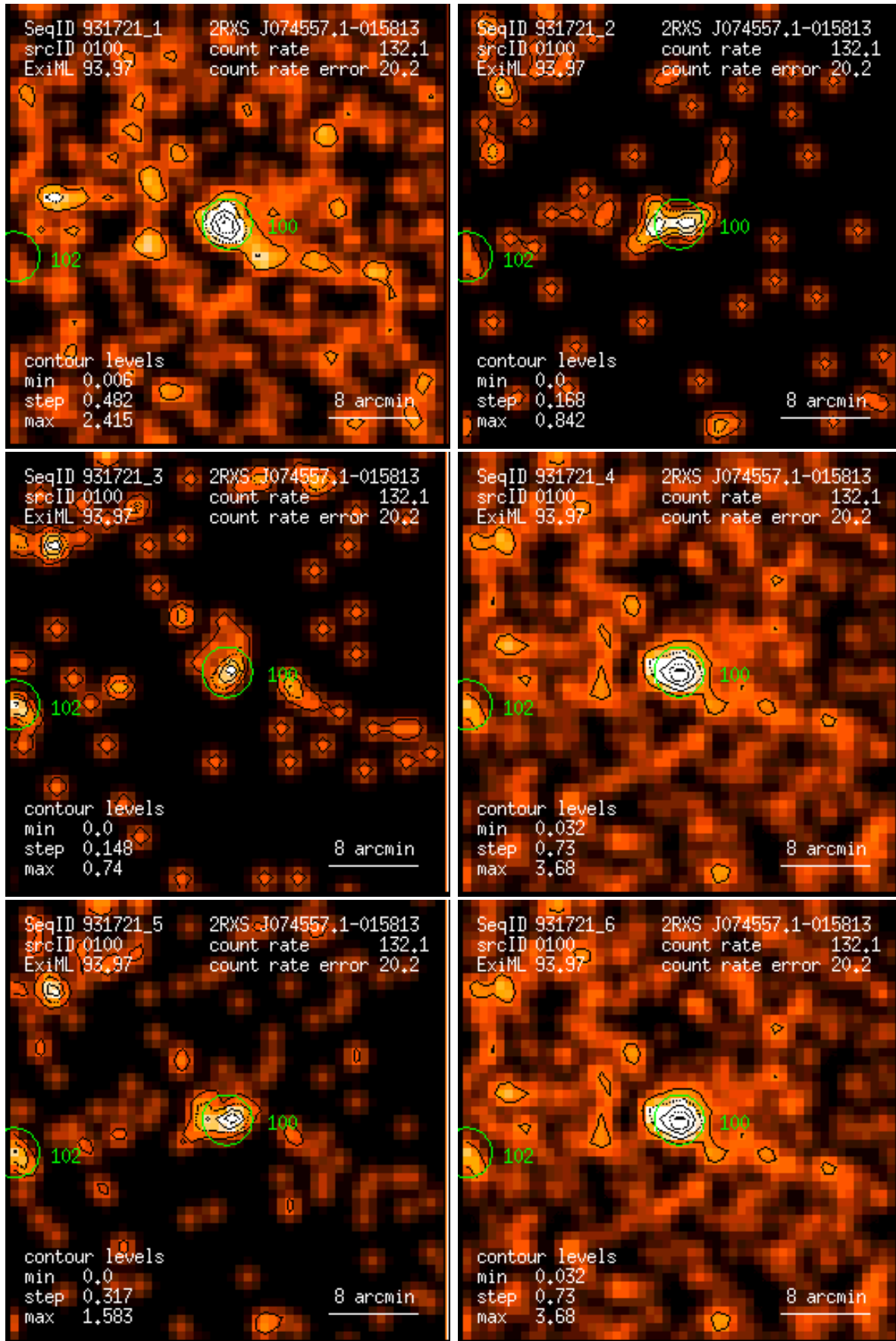
Figure 100: RASS 931721: detection 0100: band rate images, Gaussian filter: (1) PSPC channels 11 – 41, (2) 52 – 90, (3) 91 – 201, (4) 11 – 235, (5) 52 – 201, (6) 11 – 201. Broad band rates in counts/ks. Band rate contour levels in counts/ks/arcmin 2 .
