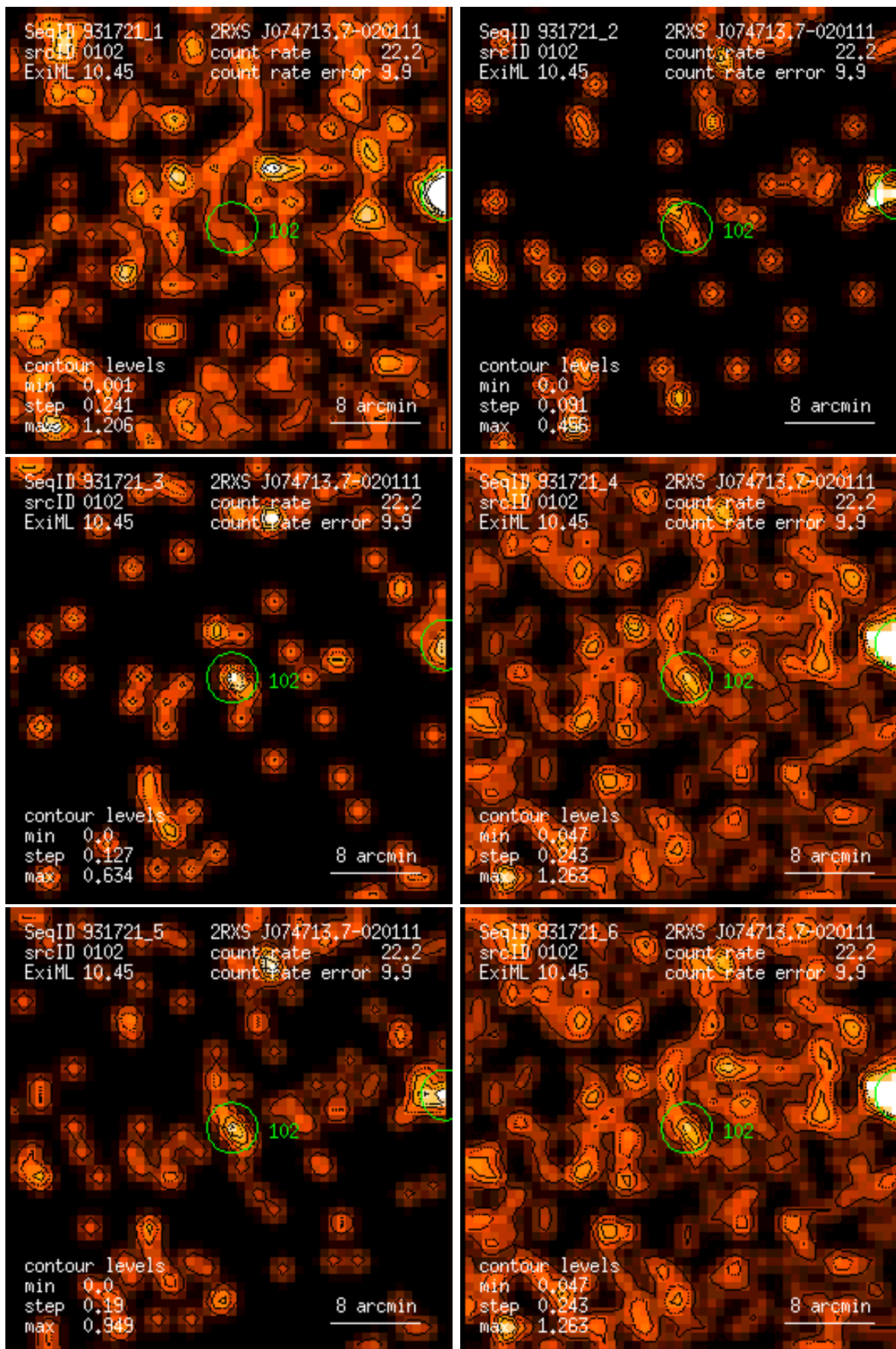
Figure 102: RASS 931721: detection 0102: band rate images, Gaussian filter: (1) PSC channels 11 – 41, (2) 52 – 90, (3) 91 – 201, (4) 11 – 235, (5) 52 – 201, (6) 11 – 201. Broad band rates in counts/ks. Band rate contour levels in counts/ks/arcmin 2 .
