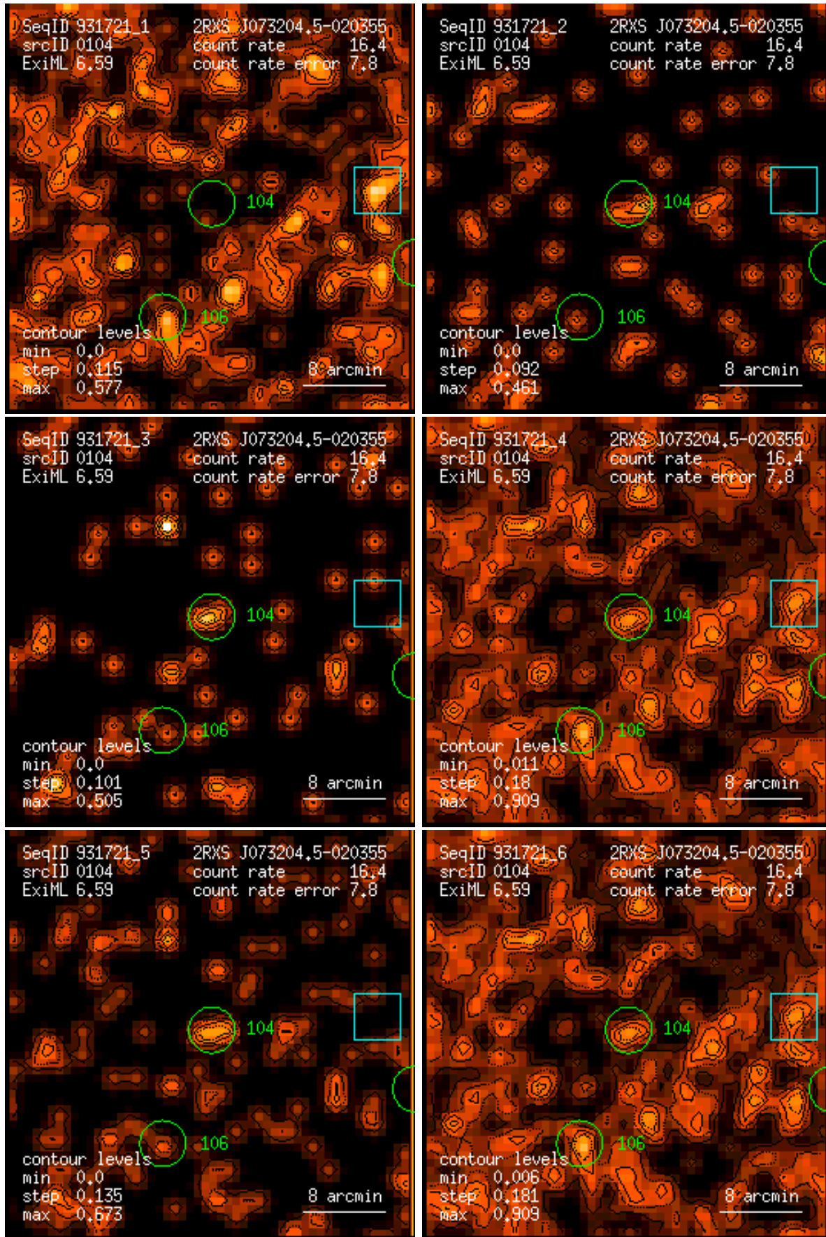
Figure 104: RASS 931721: detection 0104: band rate images, Gaussian filter: (1) PSPC channels 11 – 41, (2) 52 – 90, (3) 91 – 201, (4) 11 – 235, (5) 52 – 201, (6) 11 – 201. Broad band rates in counts/ks. Band rate contour levels in counts/ks/arcmin 2 .
