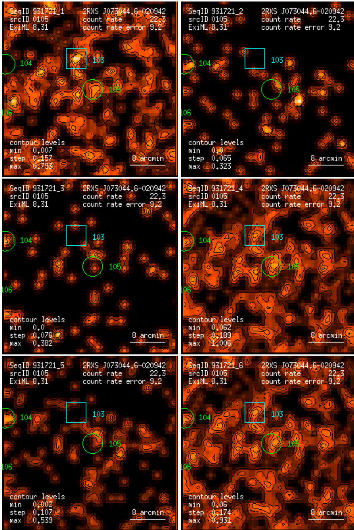
Figure 105: RASS 931721: detection 0105: band rate images, Gaussian filter: (1) PSPC channels 11 – 41, (2) 52 – 90, (3) 91 – 201, (4) 11 – 235, (5) 52 – 201, (6) 11 – 201. Broad band rates in counts/ks. Band rate contour levels in counts/ks/arcmin 2 .
