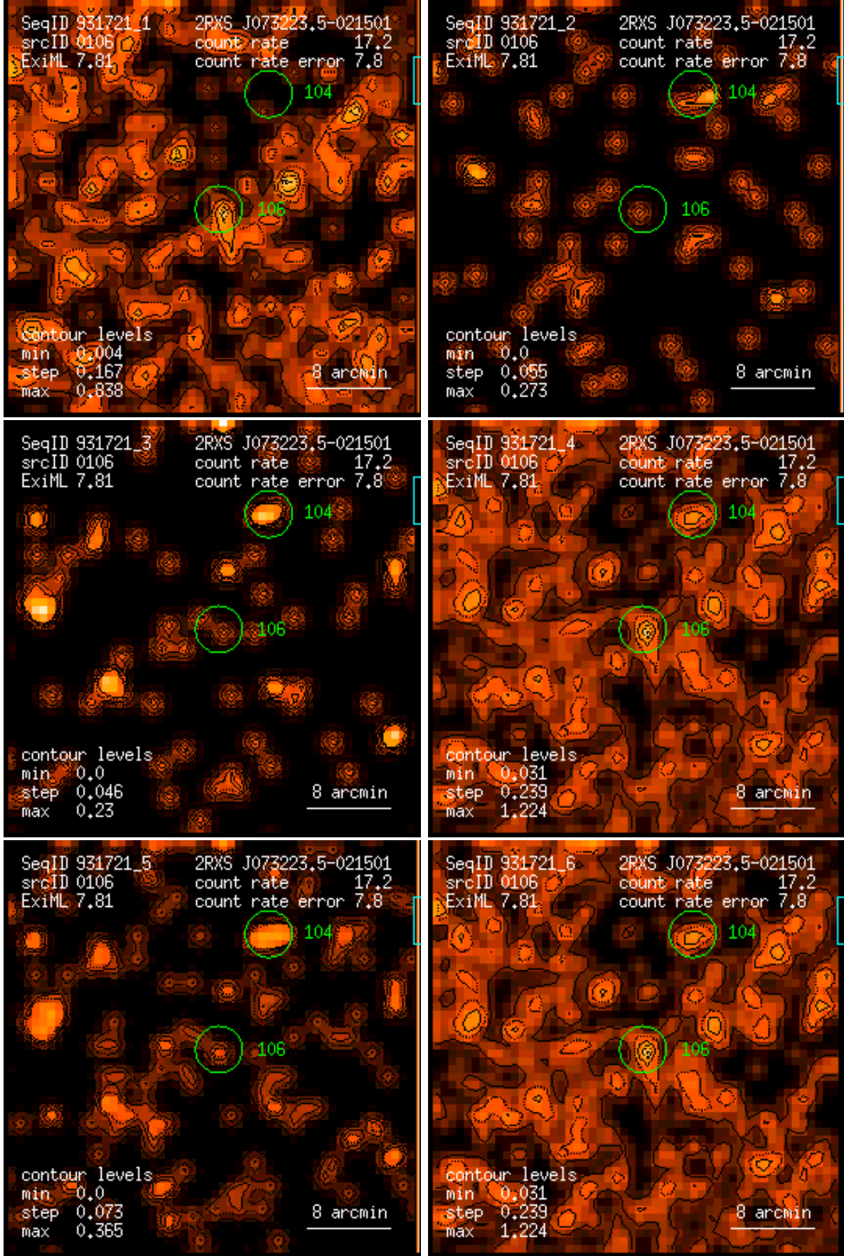
Figure 106: RASS 931721: detection 0106: band rate images, Gaussian filter: (1) PSPC channels 11 – 41, (2) 52 – 90, (3) 91 – 201, (4) 11 – 235, (5) 52 – 201, (6) 11 – 201. Broad band rates in counts/ks. Band rate contour levels in counts/ks/arcmin 2 .
