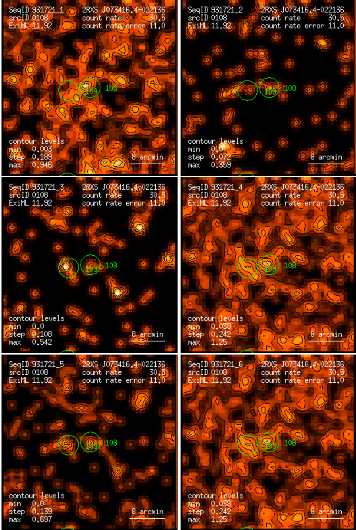
Figure 108: RASS 931721: detection 0108: band rate images, Gaussian filter: (1) PSPC channels 11 – 41, (2) 52 – 90, (3) 91 – 201, (4) 11 – 235, (5) 52 – 201, (6) 11 – 201. Broad band rates in counts/ks. Band rate contour levels in counts/ks/arcmin 2 .
